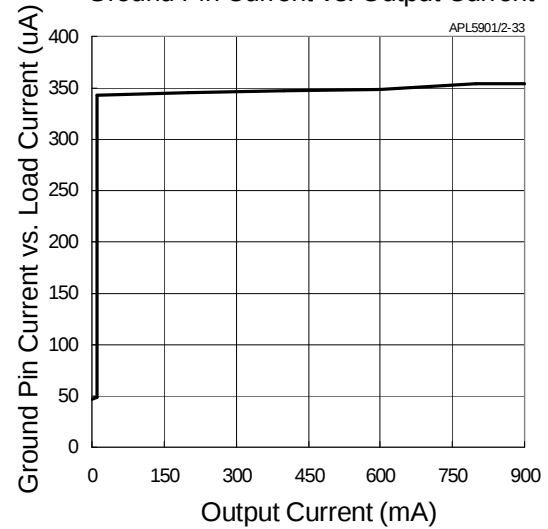
Ground Pin Current vs. Output Current
