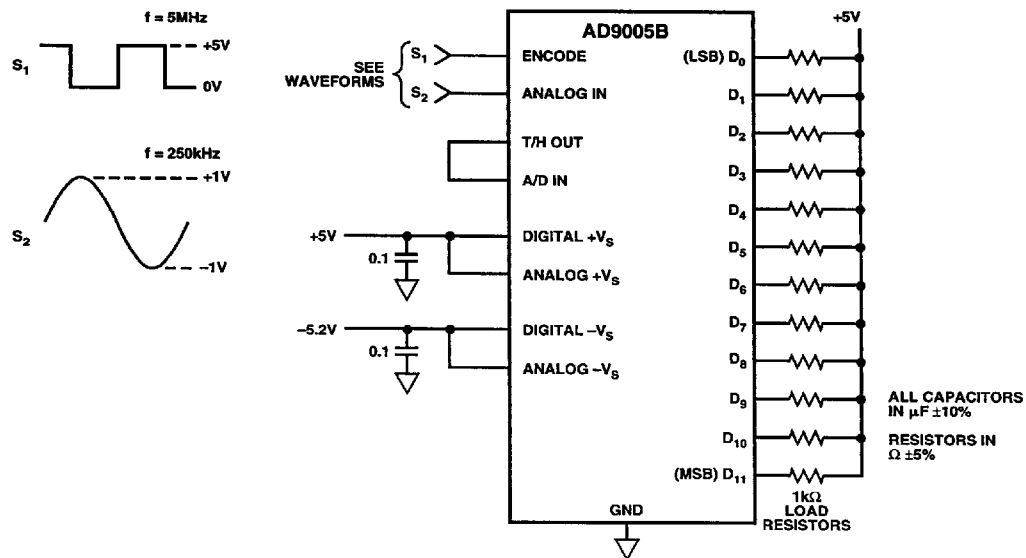
Figure 3. Burn-In Circuit
