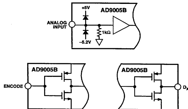
Figure 2. Equivalent Input/Output Circuits
