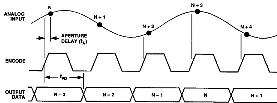
Figure 1. Timing Diagram
