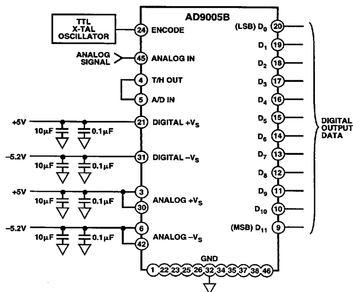
Figure 4. Typical Application
