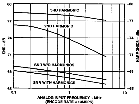
Figure 9. Dynamic Performance (@ +25°C)
