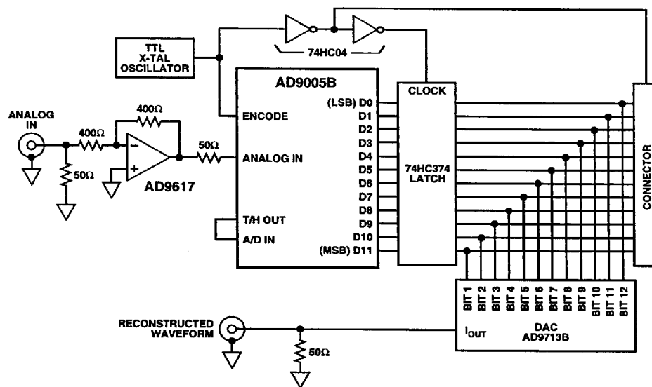
Figure 8. Evaluation Circuit
