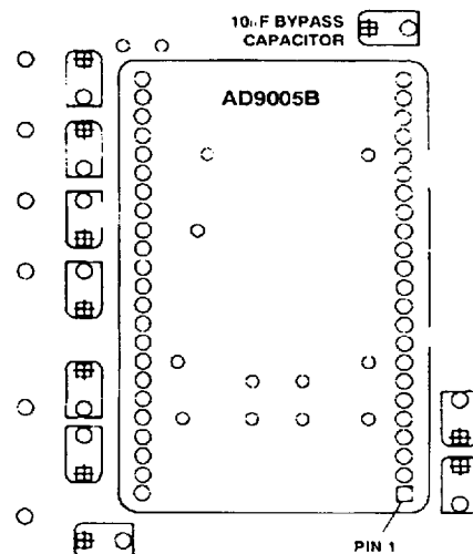
Figure 7. Component Mounting (As Viewed from Top)
