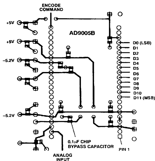
Figure 6. Solder Side (As Viewed from Top)
