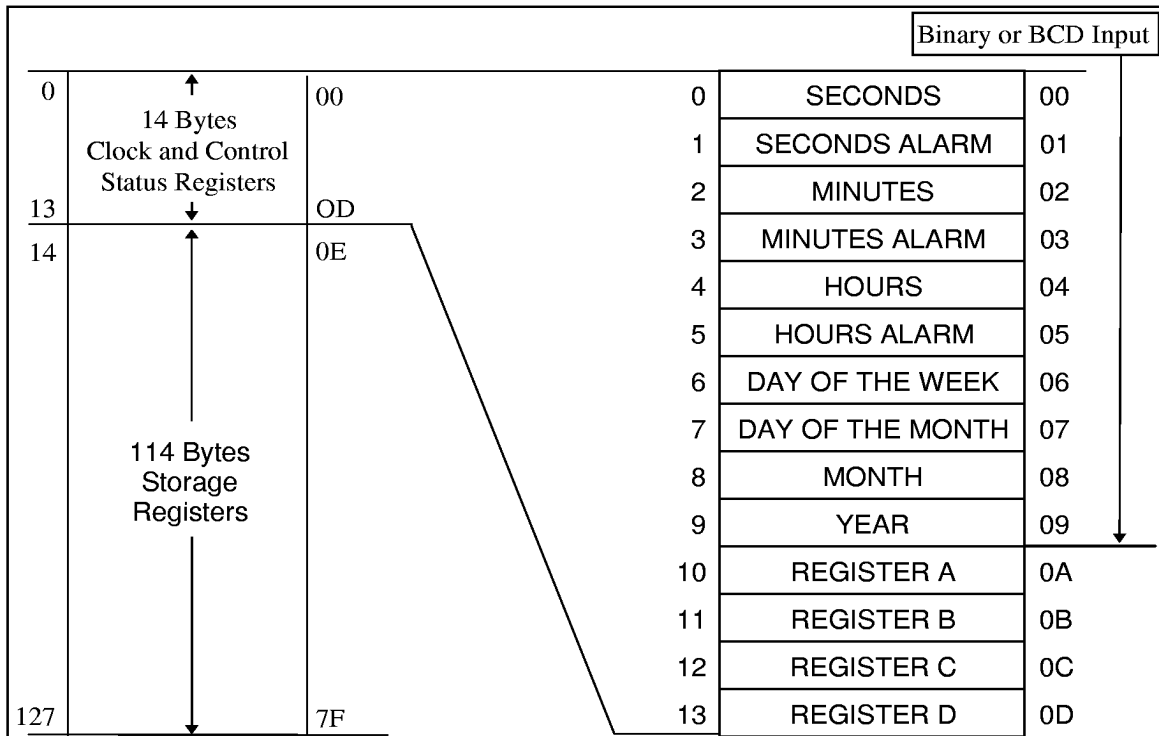
FIGURE 2: ADDRESS MAP VT82885
