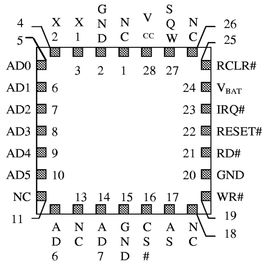
VT82885 28-PIN PLCC
