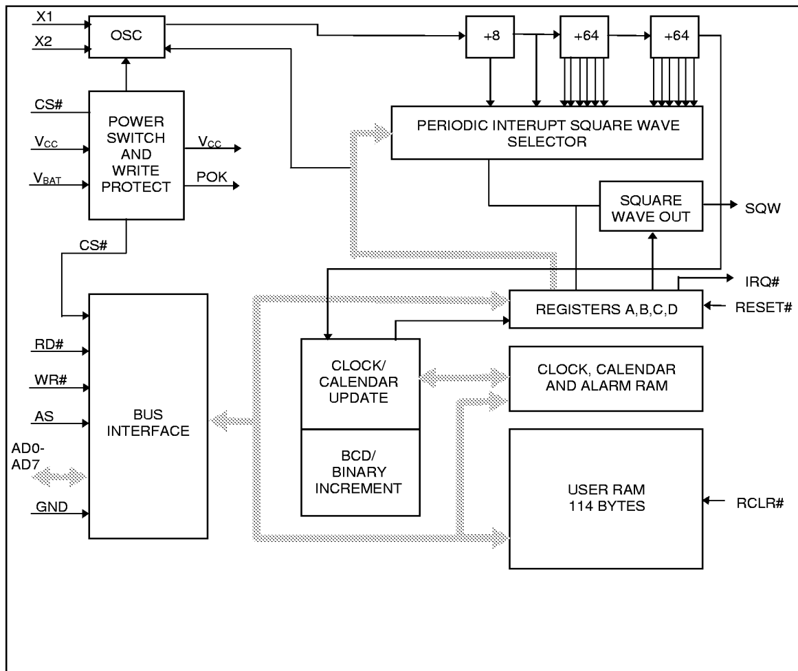
FIGURE 1: BLOCK DIAGRAM VT82885
