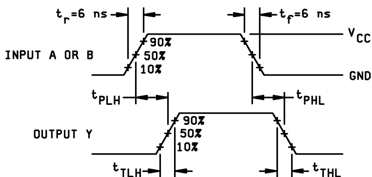
FIGURE 4. Switching waveforms and test circuit.
