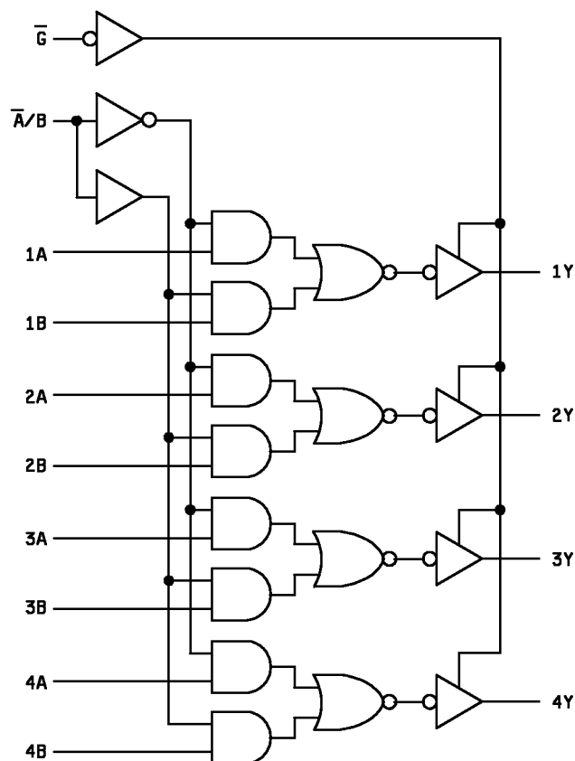
FIGURE 3. Logic diagram.
