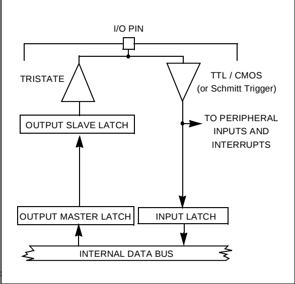
Figure 59. Input Configuration
