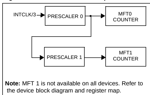
Figure 69. Parallel Mode Description
