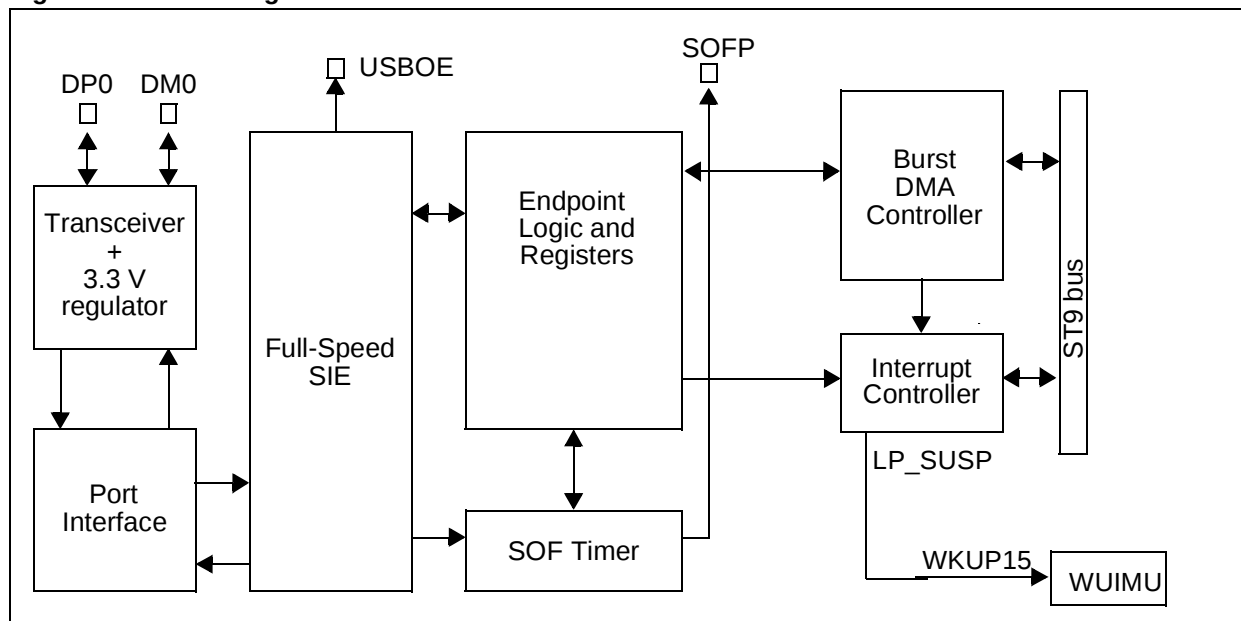
Figure 72. Block Diagram
