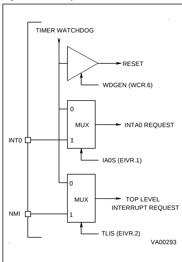
Figure 66. Interrupt Sources
