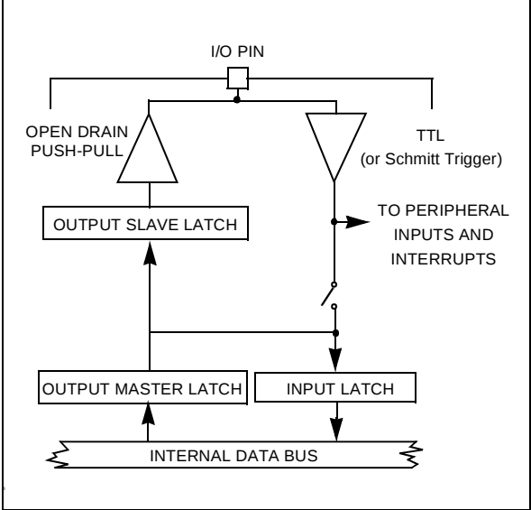
Figure 60. Output Configuration
