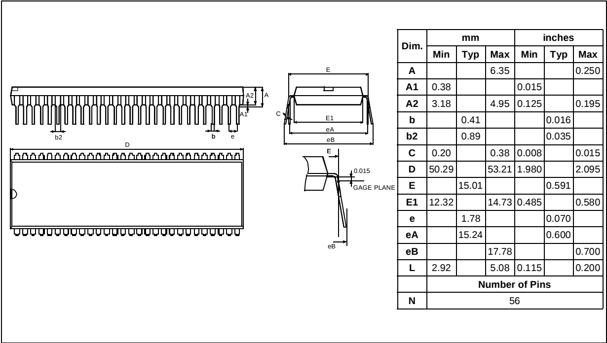
Figure 92. 56-Pin Plastic Dual In-Line Package, Shrink 600-mil Width
