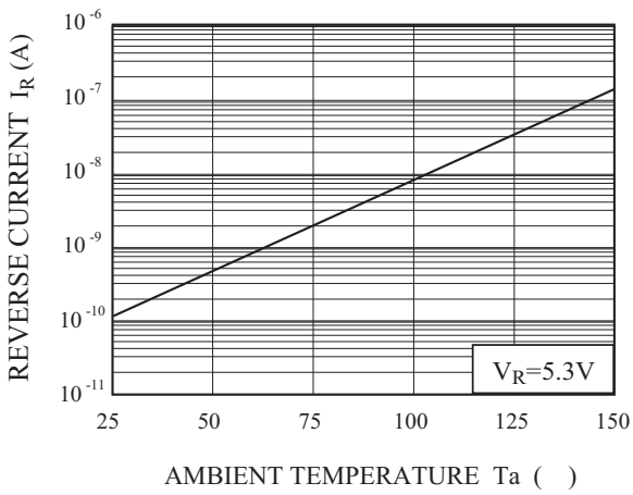
REVERSE CURRENT
