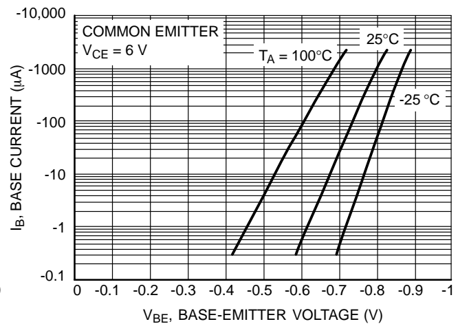
Figure 6. Base-Emitter Voltage
