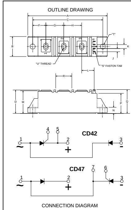
CD42__40, CD47__40 Dual SCR / Diode Isolated POW-R-BLOK™ Module 40 Amperes / Up to 1600 Volts
