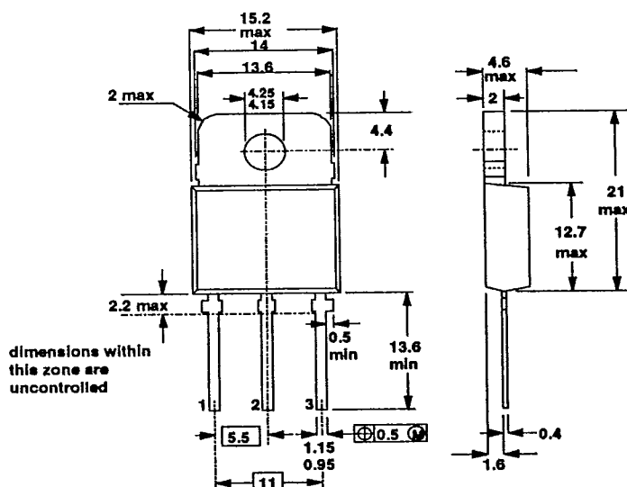
Fig.1 SOT-93; drain connected to mounting base.
