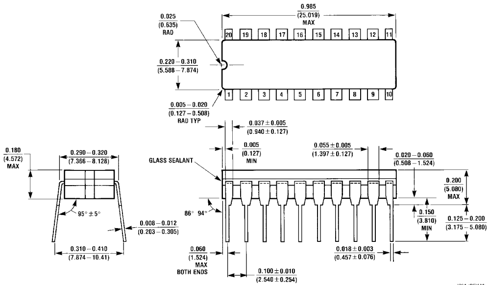
20-Lead Ceramic Dual-In-Line Package Number J20A
