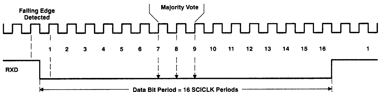
Figure 22. Asynchronous Mode
