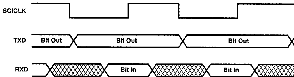
Figure 23. Isosynchronous Mode
