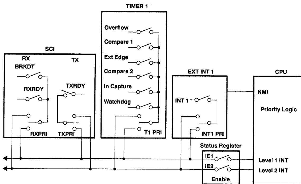
Figure 6. Interrupt Control
