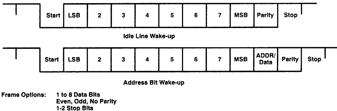
Figure 21. Frame Formats
