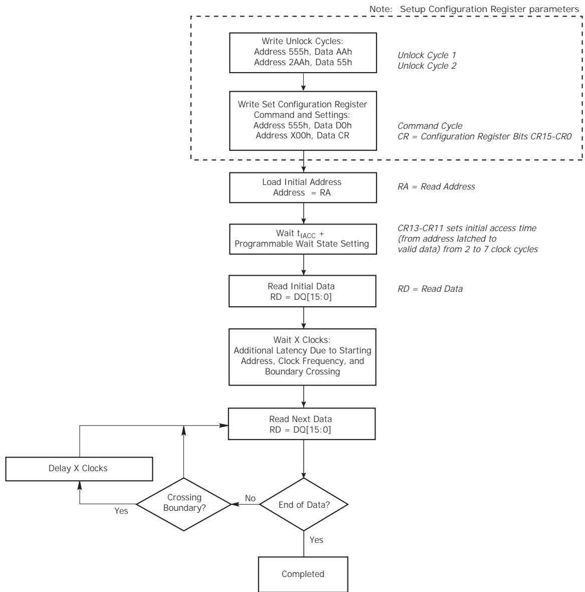
Figure 8.2 Synchronous Read
