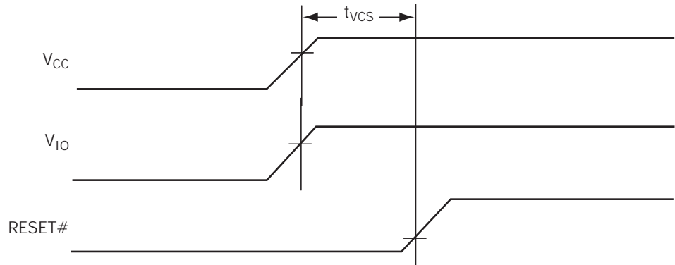
Figure 12.5 V CC Power-up Diagram
