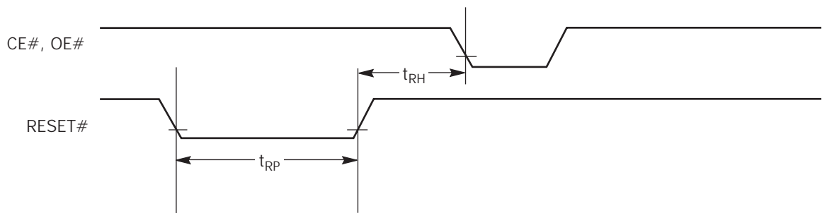
Figure 12.12 Reset Timings
