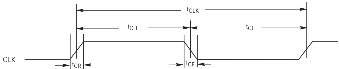
Figure I2.6 CLK Characterization
