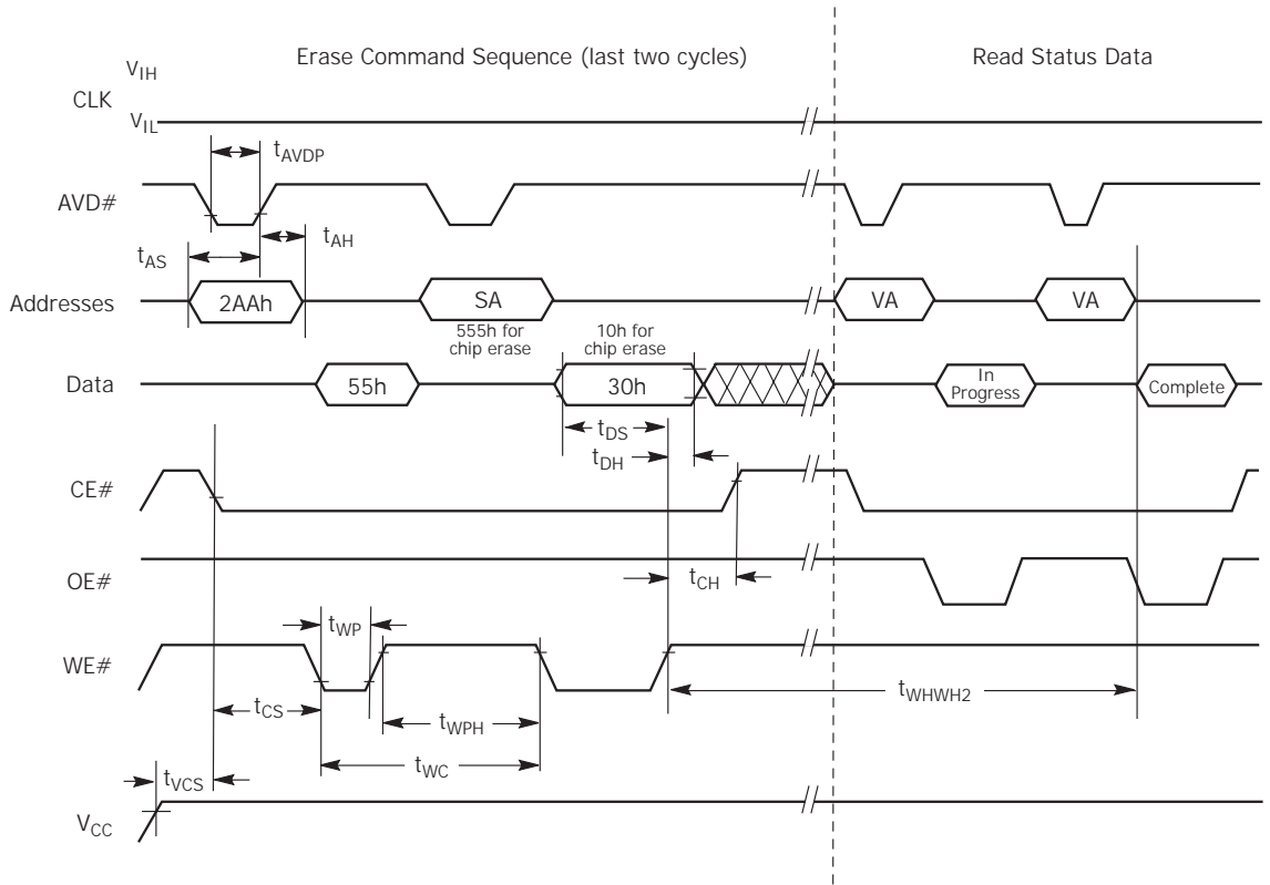
Figure I2.13 Chip/Sector Erase Operation Timings
