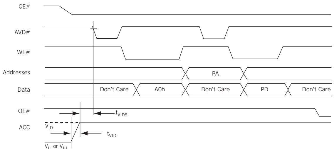
Figure I2.I6 Accelerated Unlock Bypass Programming Timing
