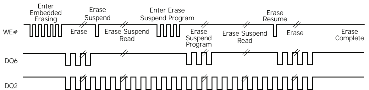
Figure 12.19 Synchronous Data Polling Timings/Toggle Bit Timings
