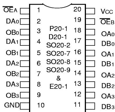
DIP/SOIC/SSOP/QSOP/ TSSOP/CERPACK TOP VIEW
