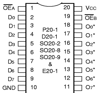
DIP/SOIC/QSOP/ TSSOP/CERPACK TOP VIEW
