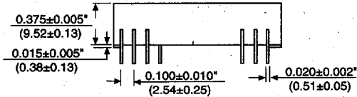
SIDE VIEWS
