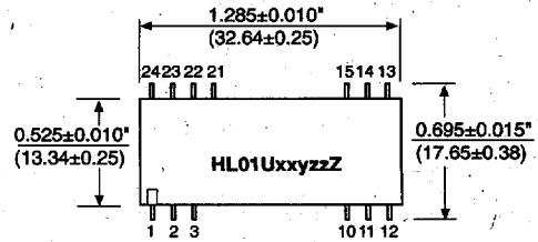
TOP VIEWS
