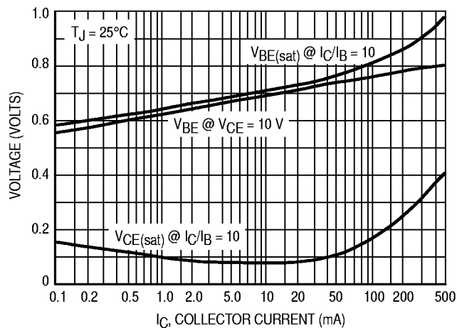
Figure 17. "On" Voltages
