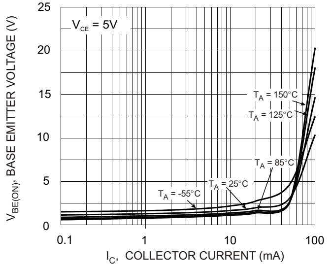
Fig. 17 V BE(ON) vs I C
