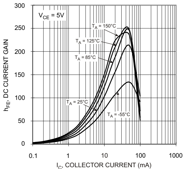
Fig. 13 DC Current Gain
