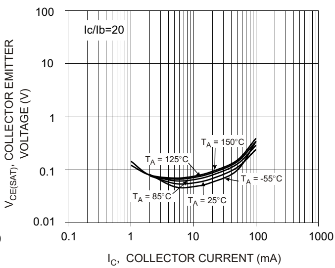
Fig. 15 V_{CE(SAT)} vs I_C
