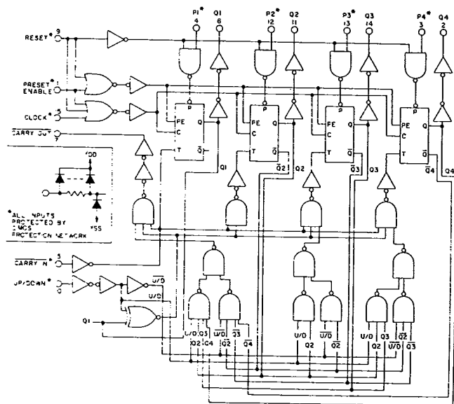
Fig. 10 — Logic Diagram for CD4510B.
