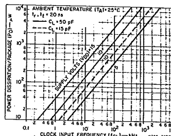
Fig. 9 — Typical dynamic power dissipation vs. frequency.
