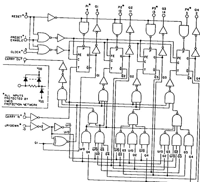
Fig.3 - Logic Diagram for CD4510B.
