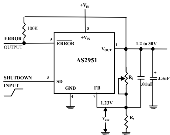
Figure 2. Adjustable Regulator
