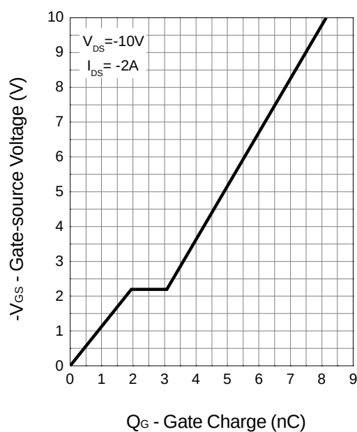
Gate Charge
