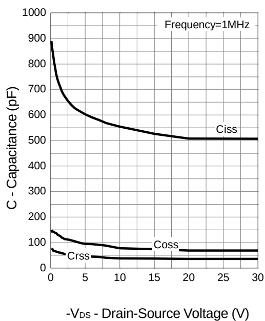
Capacitance
