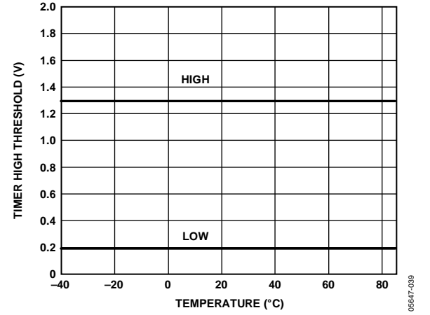
Figure 14. Timer Threshold vs. Temperature
