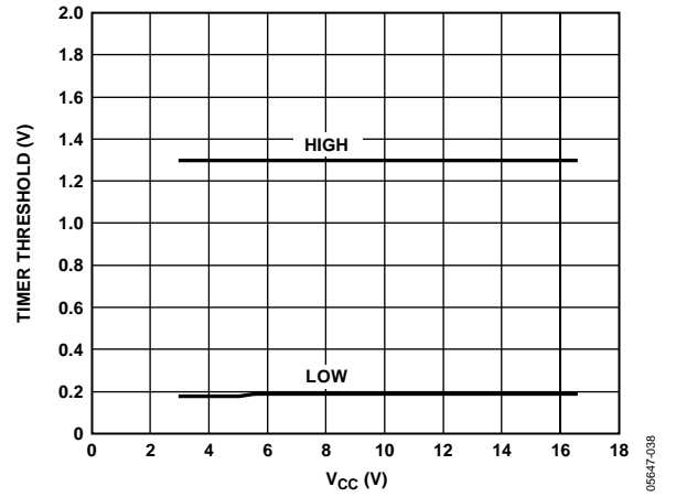
Figure 13. Timer Threshold vs. Supply Voltage
