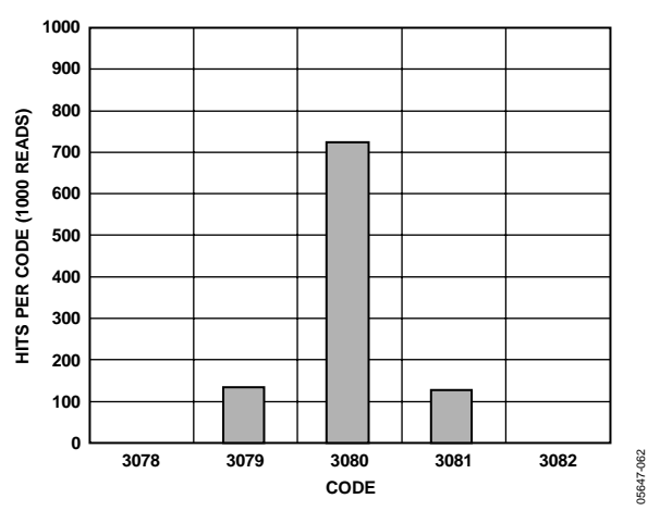
Figure 27. ADC Noise, 7:1 Voltage Channel, 5 V Input, 1000 Reads
