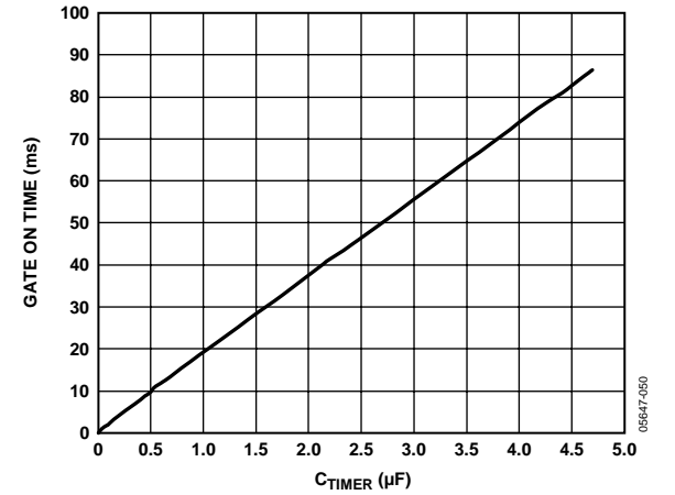
Figure 15. Current Limit On Time vs. Timer Capacitance
