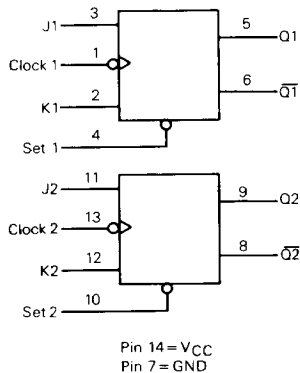
LOGIC DIAGRAM
