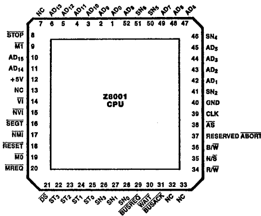
Figure 10b. 52-pin Chip Carrier, Pin Assignments
