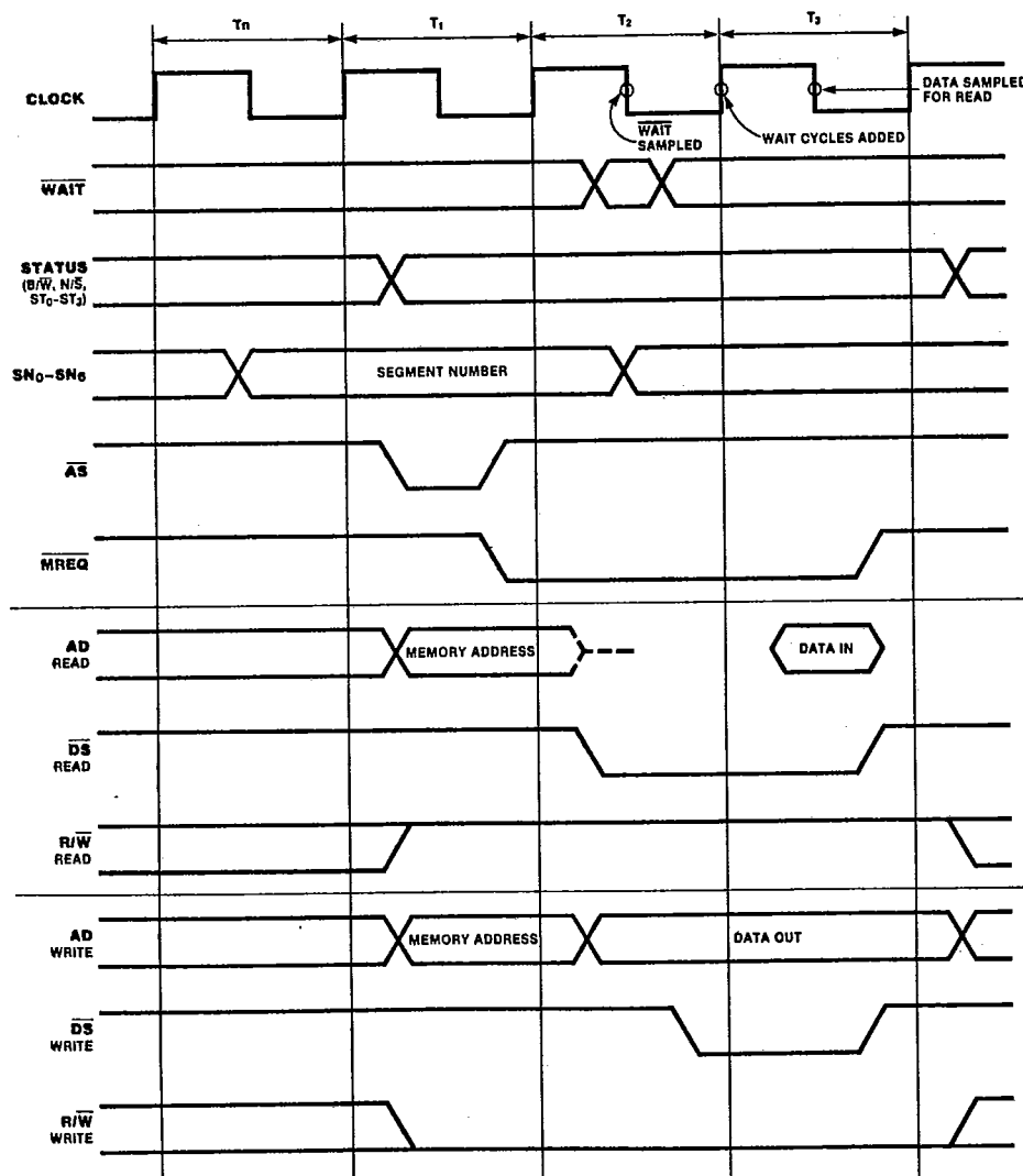
Figure 1. Memory Read and Write Timing
