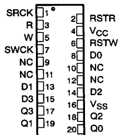
SD PACKAGE† (TOP VIEW)
