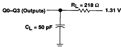
Figure 1. Load Circuit for Timing Parameters
