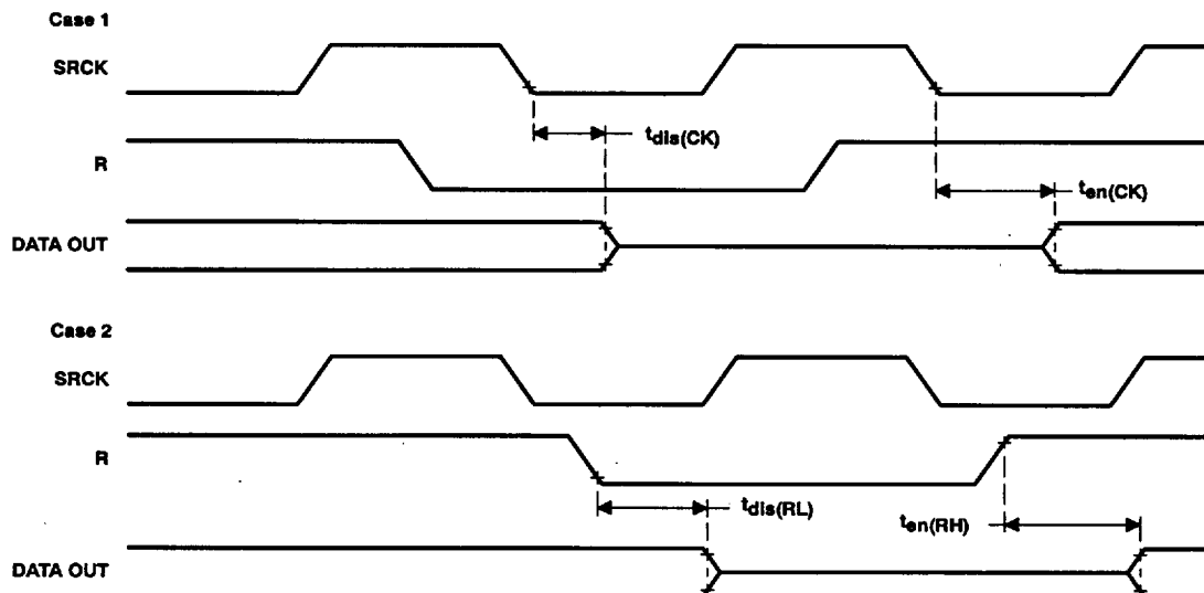
Figure 6. Read Cycle Timing (Output Enable and Disable)
