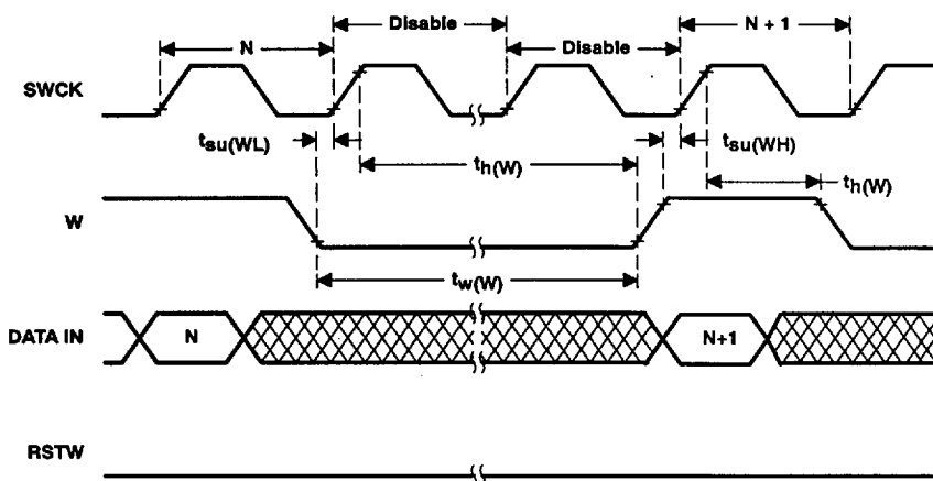
Figure 3. Write Cycle Timing (Write Enable)
