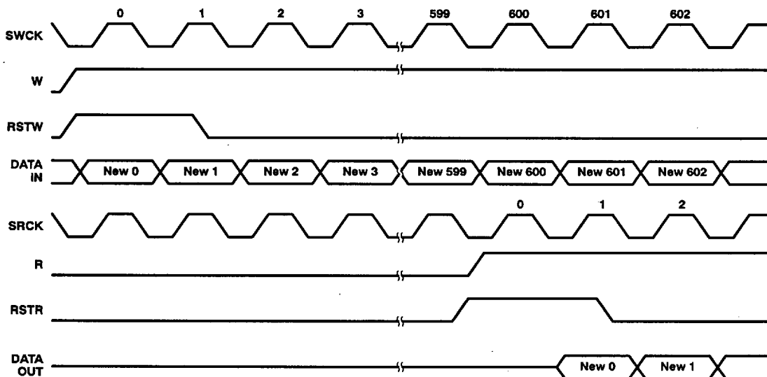
Figure 7. New Data Access Mode
