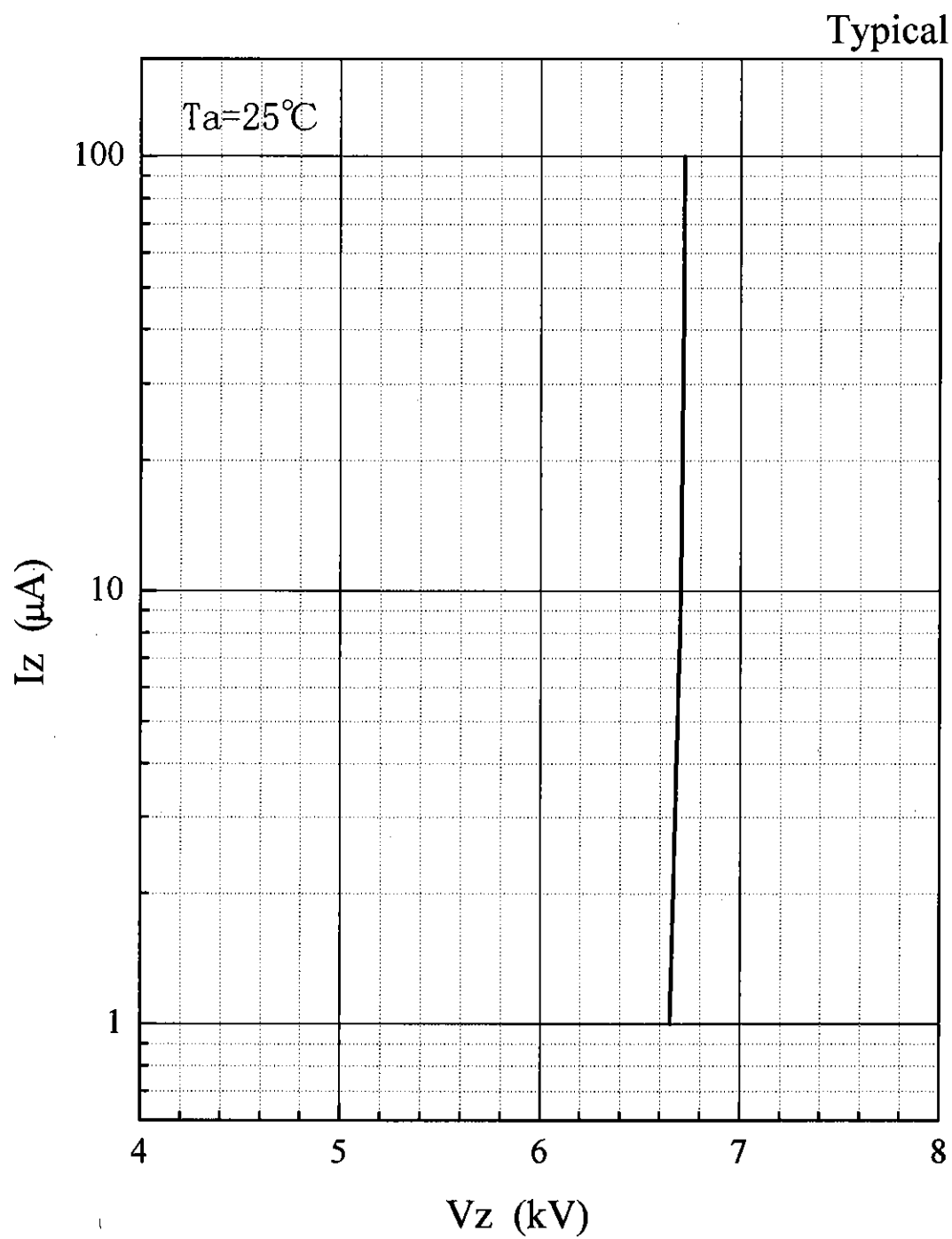
Fig.3 Avalanche characteristic [ V_z - I_z ]
