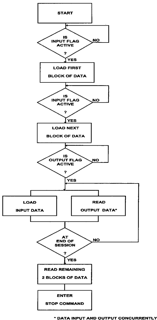
Figure 3-23 : Pipelining Operational Flow Chart
