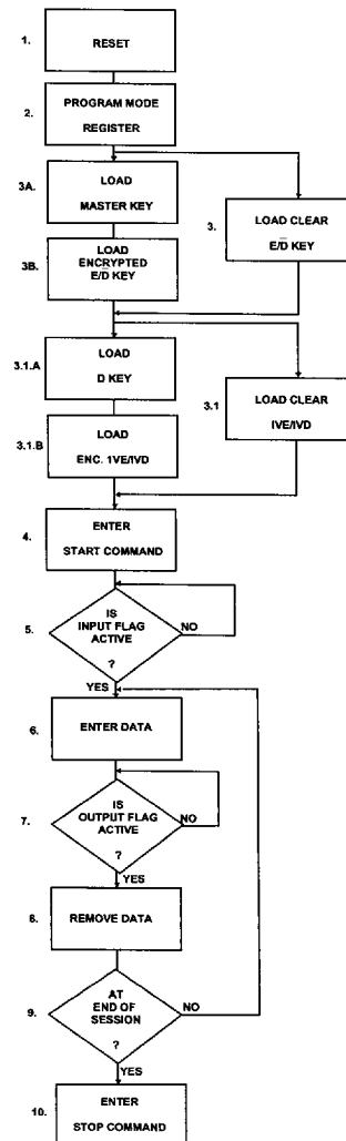
Figure 3-19 : Multiplexed Control Mode CBC Programming Flow Chart
