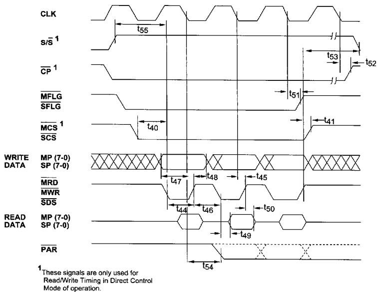
Figure 3-11 : CA95C68 Master (Slave) Port Read/Write Timing
