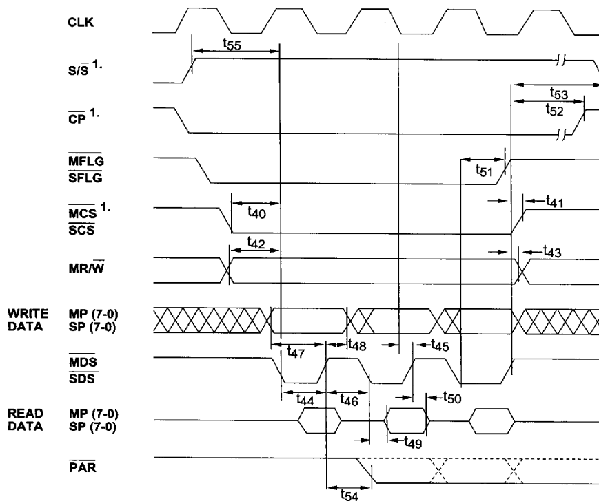
Figure 3-14 : CA95C18 Master (Slave) Port Read/Write Timing
