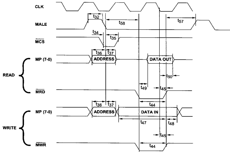
Figure 3-10 : CA95C68 Master Port, Multiplexed Control Mode Read/Write
