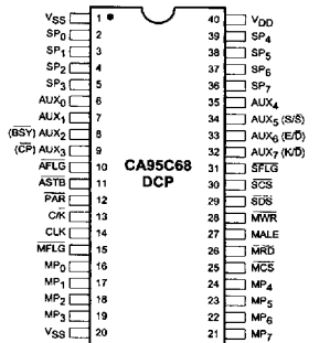
Figure 3-2 : CA95C68 40-Pin PDIP
