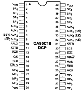
Figure 3-3 : CA95C18 40-Pin PDIP
