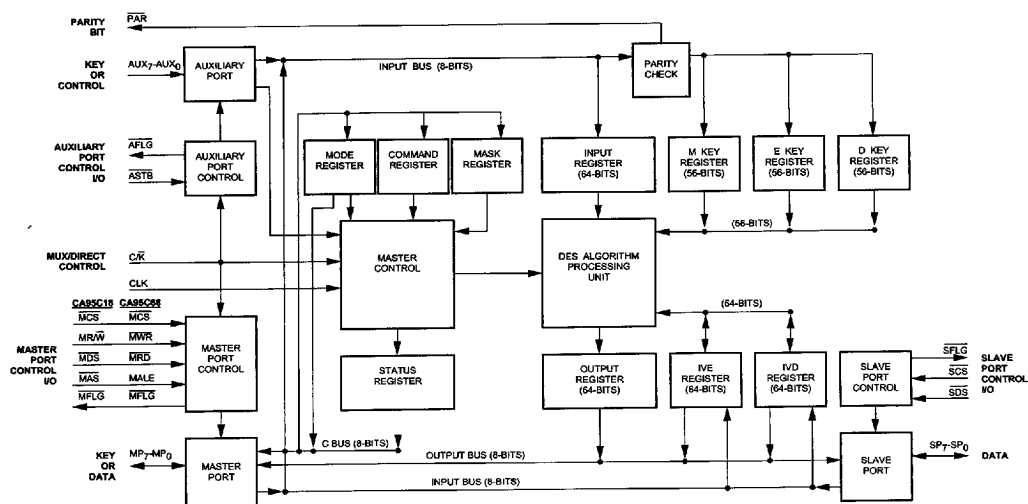
Figure 3-1 : CA95C68/18/09 Block Diagrams
