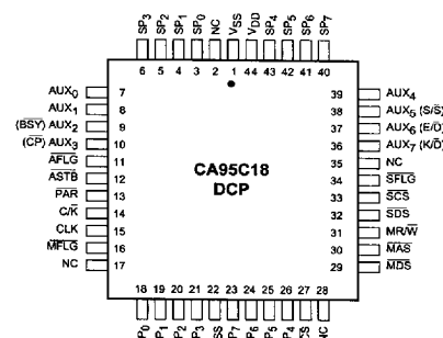
Figure 3-6 : CA95C18 44-Pin PLCC
