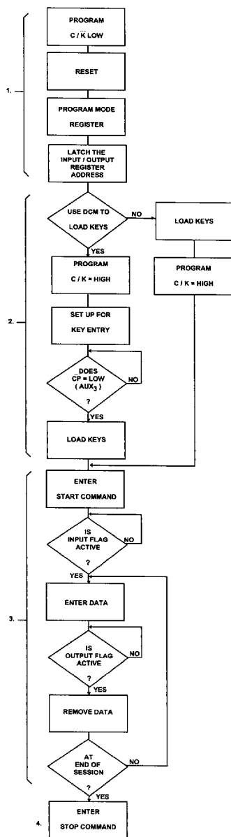
Figure 3-20 : Direct Control Mode ECB Programming Flow Chart
