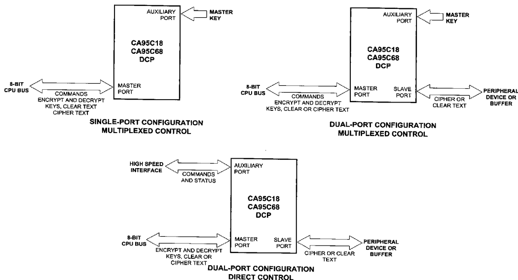
Figure 3-15: CA95C68 and CA95C18 Data Flow Options
