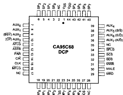
Figure 3-5 : CA95C68 44-Pin PLCC
