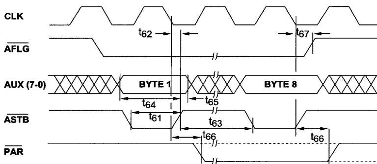
Figure 3-12 : CA95C68/18 Auxiliary - Port Key Entry Timing
