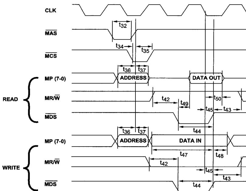
Figure 3-13 : CA95C18 Master Port, Multiplexed Control Mode, Read/Write Timing
