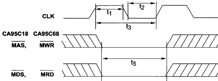
Figure 3-8 : CA95C68/18 Clock and Reset Timing
