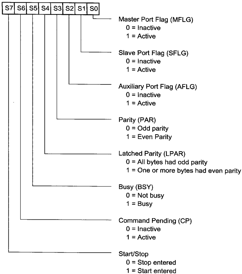
Figure 3-17 : Status Register Bit Assignments
