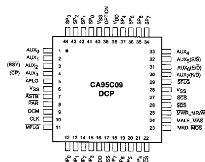
Figure 3-7 : CA95C09 44-Pin TQFP
