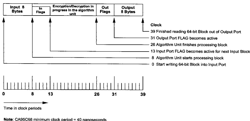
Figure 3-22 : Detailed Timing of One Block
