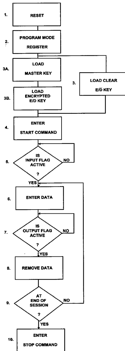
Figure 3-18 : Multiplexed Control Mode ECB Programming Flow Chart
