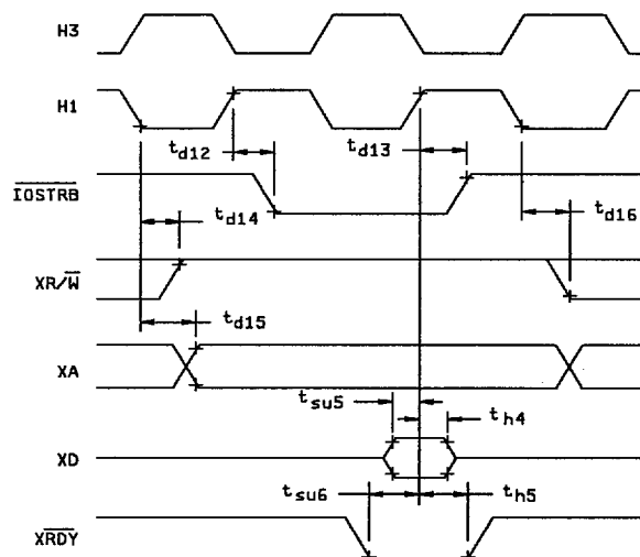
Memory ((IO)STRB = 0) Read
