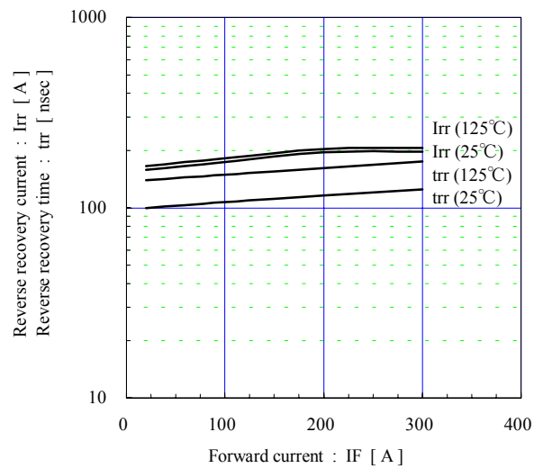
Reverse recovery characteristics (typ.) Vcc=600V, VGE=±15V, Rg=3 Ω
