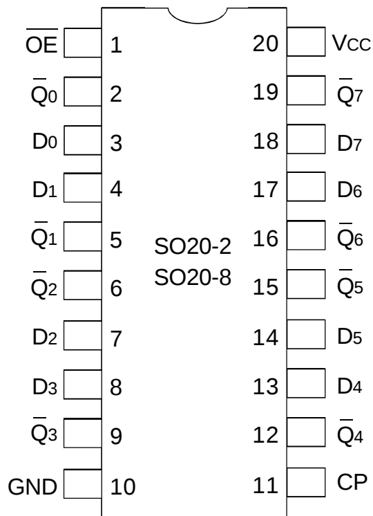
SOIC/ QSOP TOP VIEW
