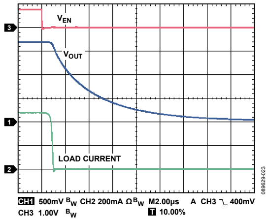
Figure 23. Typical Turn-Off Time, V IN = 1.8 V, R LOAD = 3.6 \Omega
