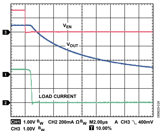
Figure 24. Typical Turn-Off Time, V IN = 3.6 V, R LOAD = 7.5 \Omega
