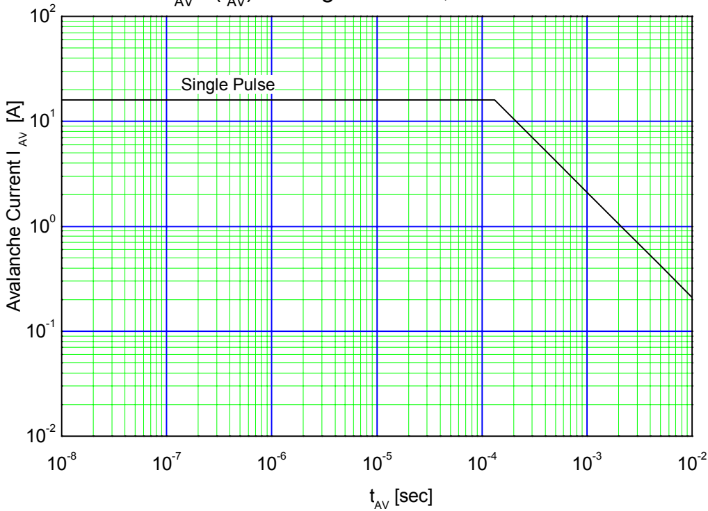
Maximum Avalanche Current Pulsewidth I_{AV}=f(t_{AV}): \text{starting Tch}=25^{\circ}C, V_{CC}=48V
