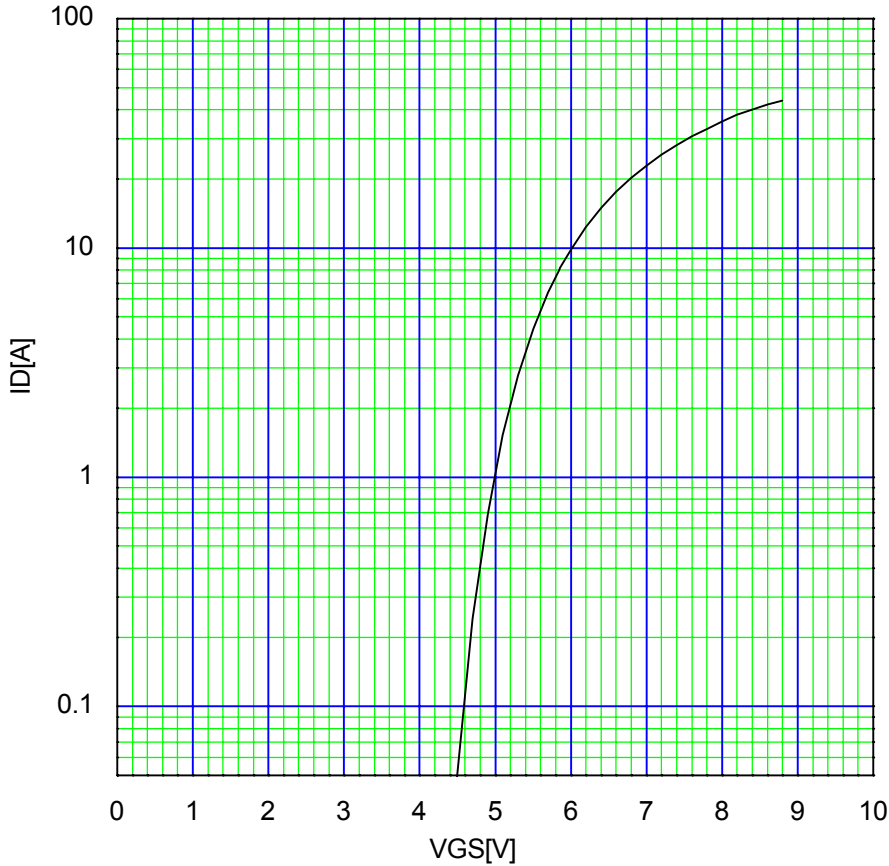
Typical Transfer Characteristic I_D=f(V_{GS}):80\text{ }\mu\text{s pulse test, }V_{DS}=25\text{V, }T_{ch}=25^\circ\text{C}
