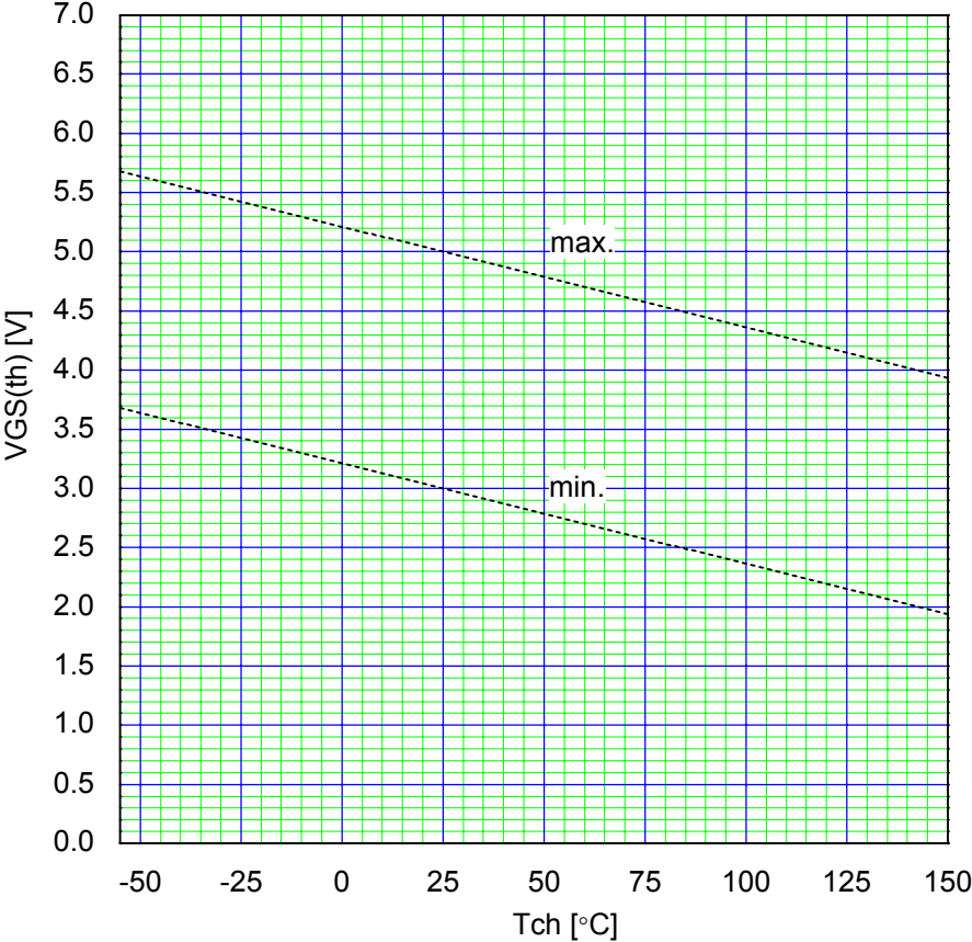
Gate Threshold Voltage vs. T ch V_{GS(th)}=f(T_{ch}):V_{DS}=V_{GS},I_D=25\mu A
