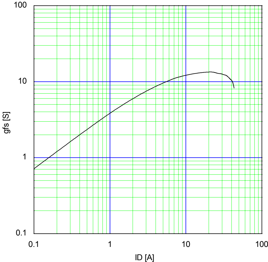
Typical Transconductance g_{fs}=f(I_D):80\text{ }\mu\text{s pulse test, }V_{DS}=25\text{V, }T_{ch}=25^\circ\text{C}
