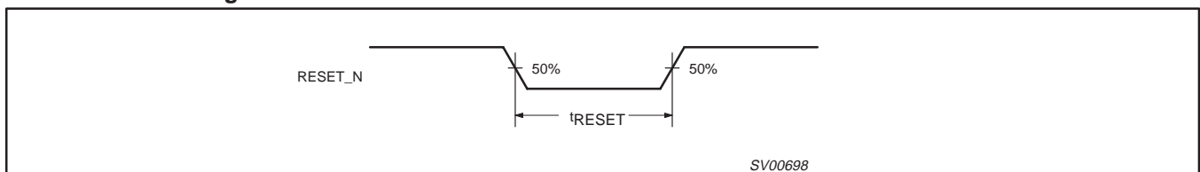
Figure 43. RESET_N Waveform
