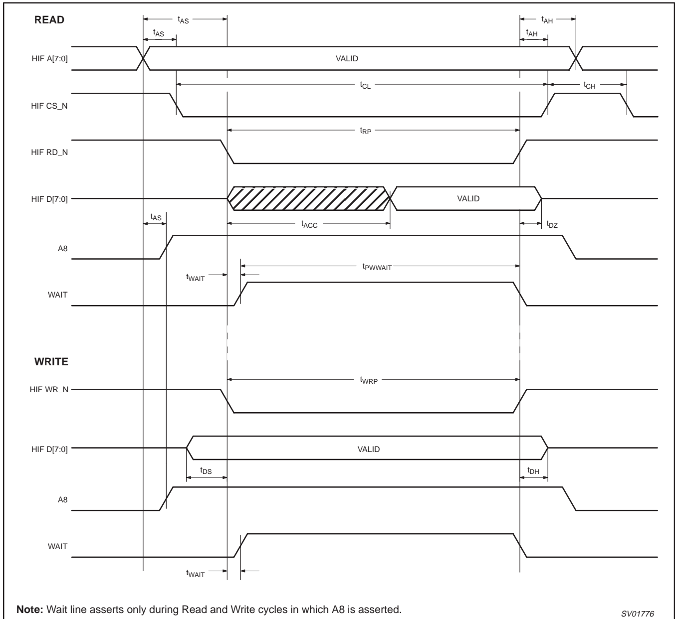
Figure 40. Host Interface Timing Waveforms
