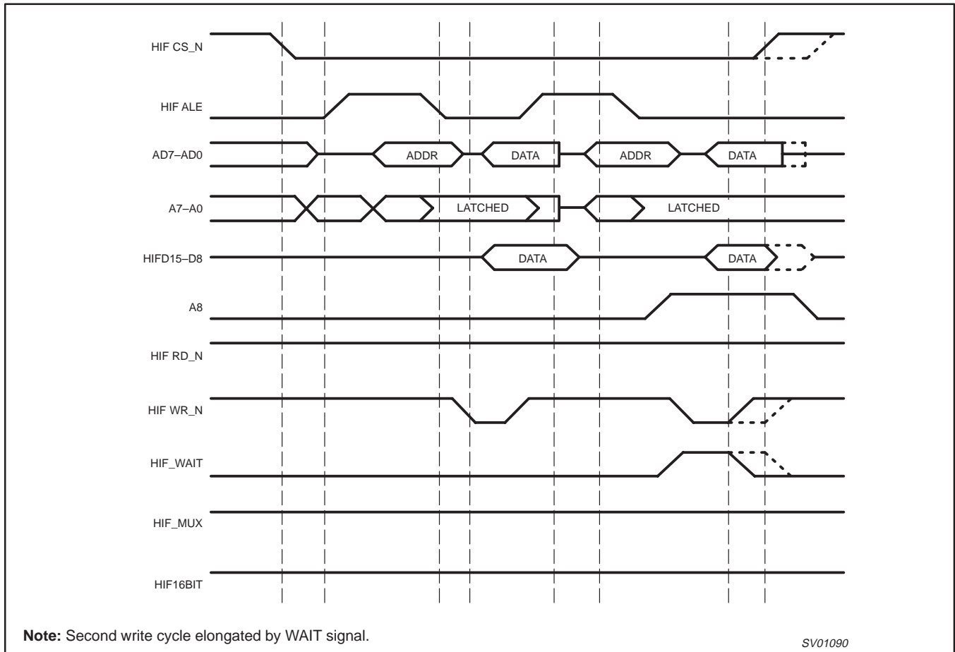
Figure 8. 16 Bit Write Cycle Multiplexed
