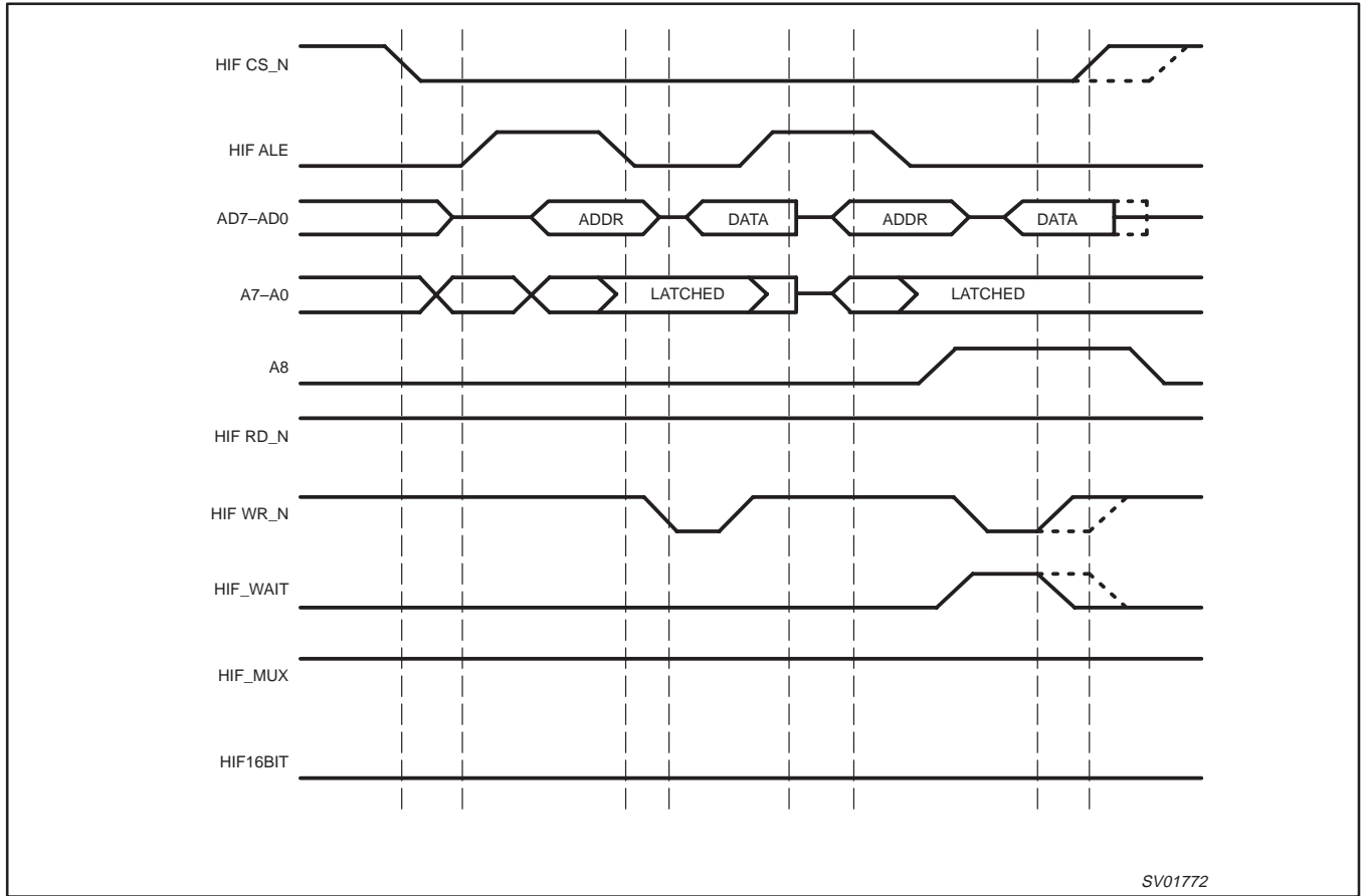
Figure 10. 8 Bit Write Cycle Multiplexed
