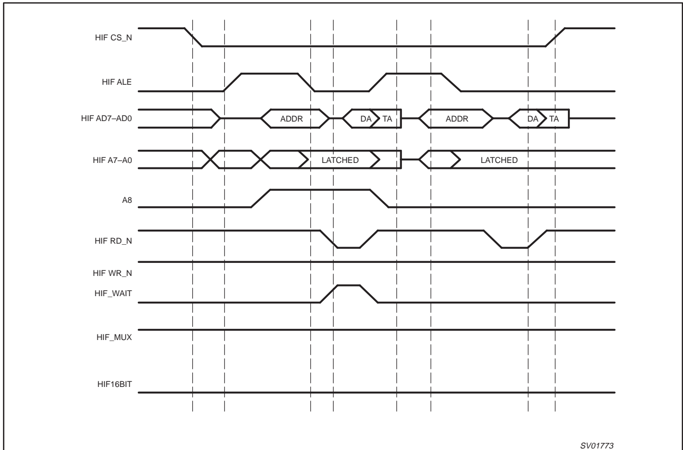
Figure 11. 8 Bit Read Cycle Multiplexed
