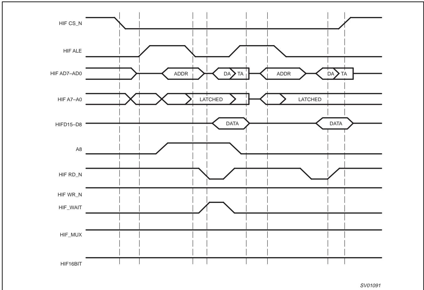
Figure 9. 16 Bit Read Cycle Multiplexed
