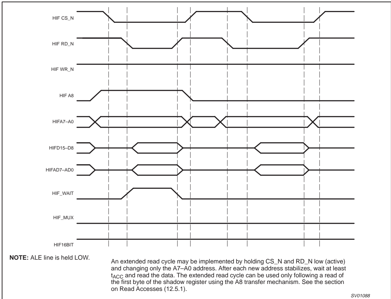
Figure 6. 16 Bit Read Cycle Non-multiplexed
