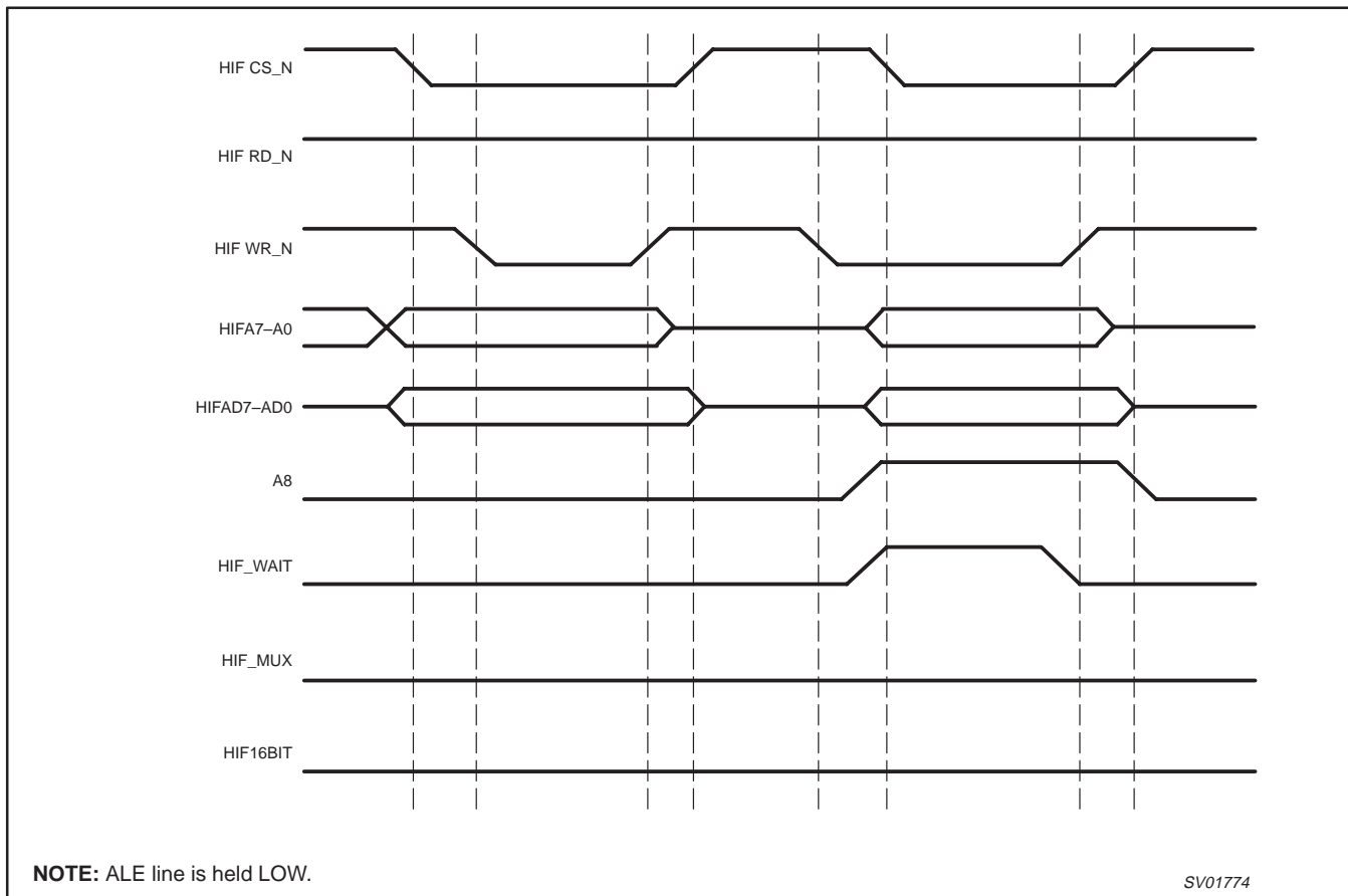
Figure 12. 8 Bit Write Cycle Non-multiplexed
