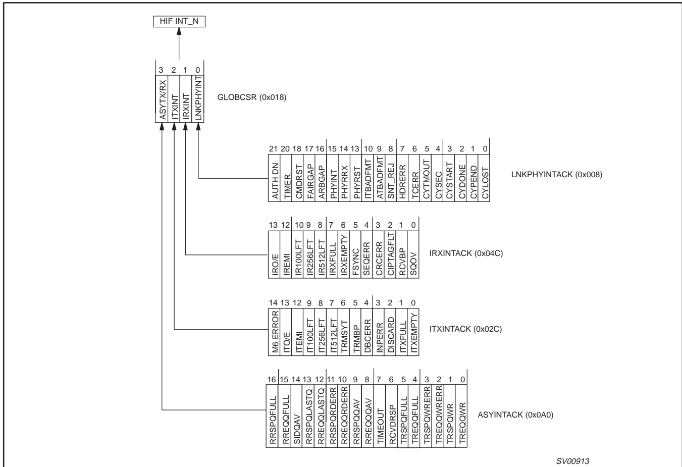
Figure 33. Interrupt Hierarchy
