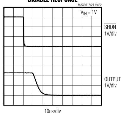
MAX9517 DISABLE RESPONSE
