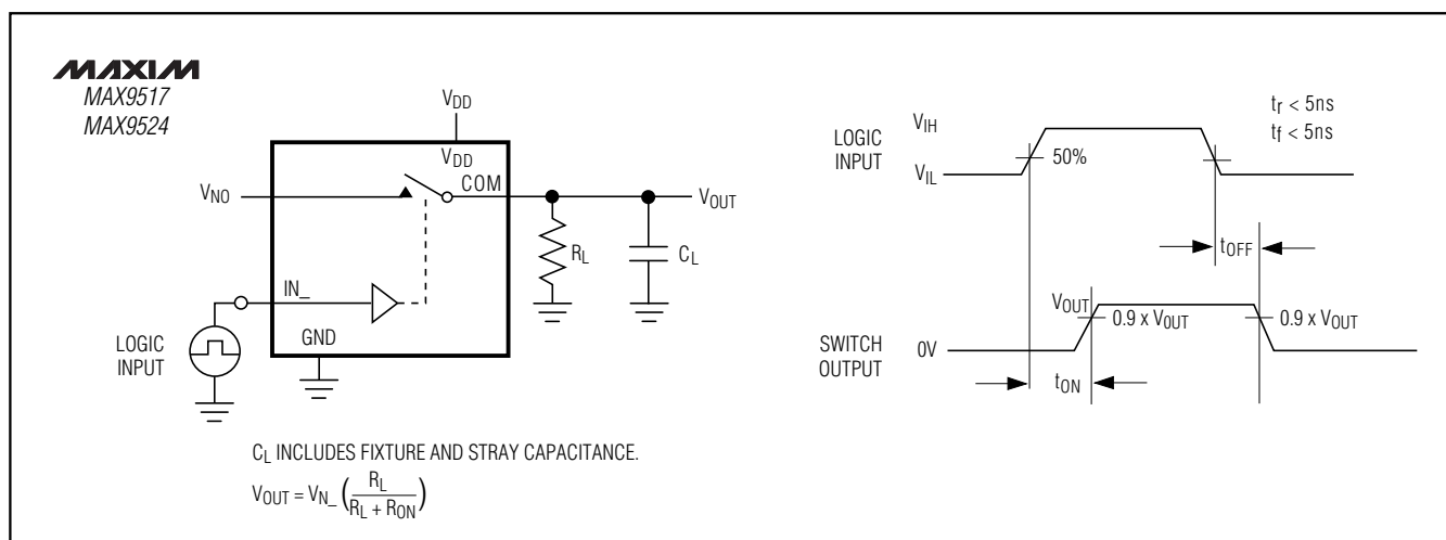
Figure 12. Switching Time
