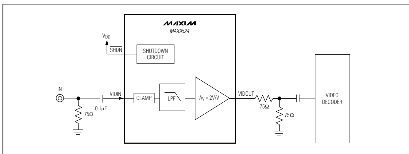
Figure 11. MAX9524 is Used as an Anti-Alias Filter with Buffer (Switches Can Route Other Signals)
