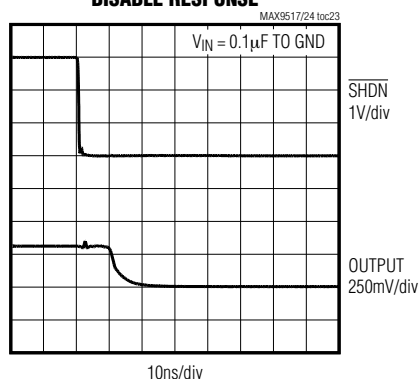
MAX9524 DISABLE RESPONSE
