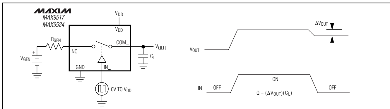
Figure 14. Charge Injection
