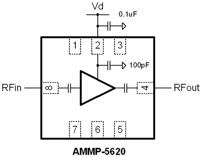
Figure 21. Typical Application.
