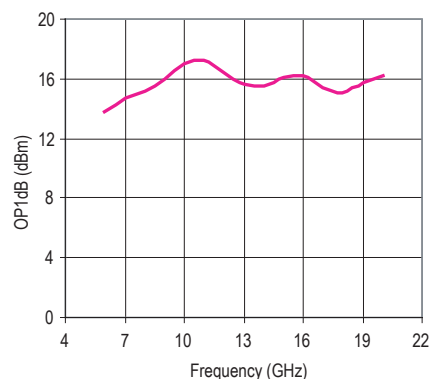
Figure 6. P1dB
