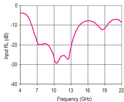
Figure 3. Input Return Loss
