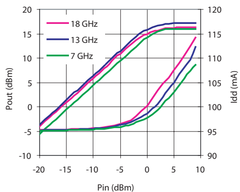
Figure 7. Pout and Idd vs. Pin
