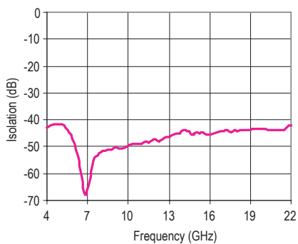
Figure 2. Isolation
