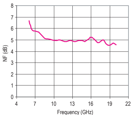
Figure 5. Noise Figure
