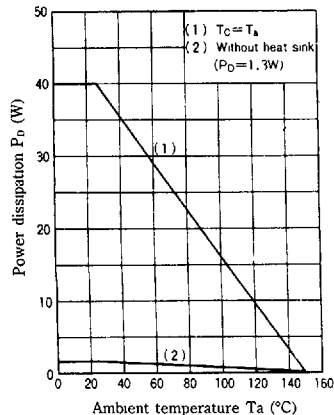
P_D - T_a
