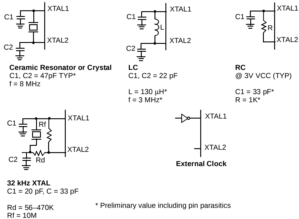
Figure 38. Oscillator Configuration
