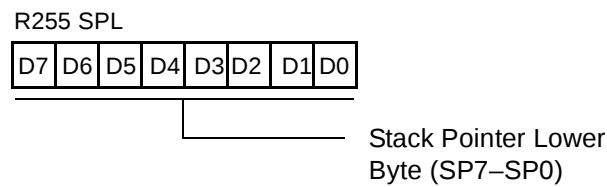
Figure 67. Stack Pointer Low—(0) FFH: Read/Write
