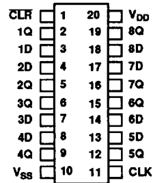
20-Lead Flatpack Top View
