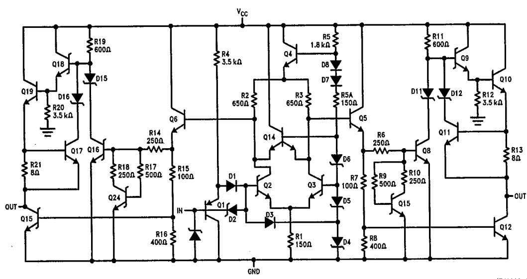
FIGURE 1. Equivalent Circuit
