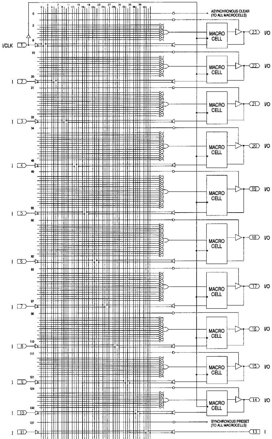
Figure 3. PEEL22CV10A Logic Array Diagram
