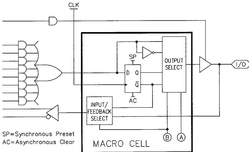
Figure 4. Block Diagram of the PEEL22CV10A I/O Macrocell
