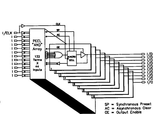
Block Diagram (Figure 2)
