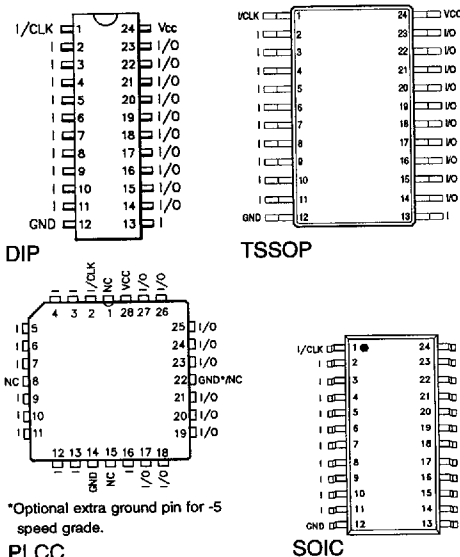
Pin Configuration (Figure 1)
