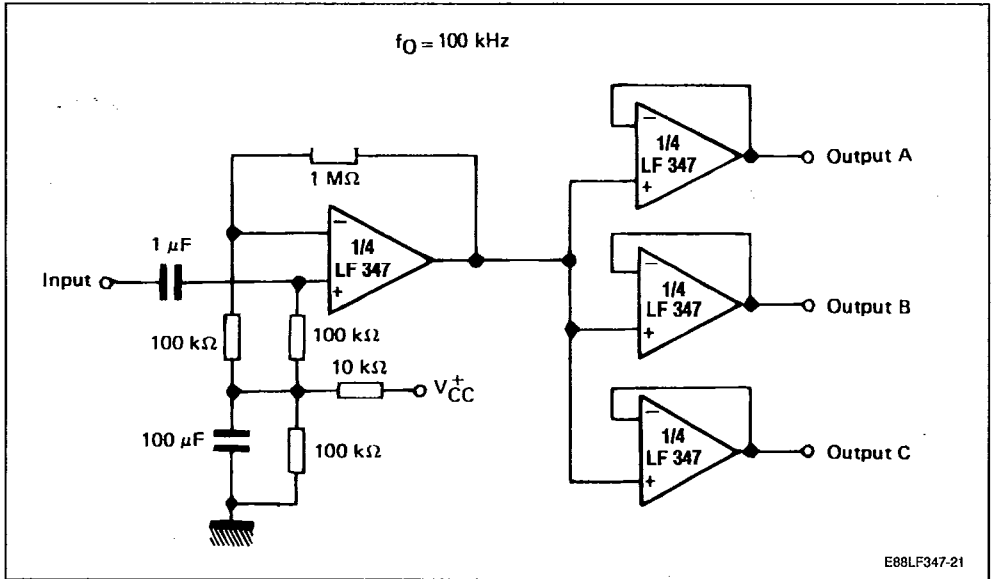
Figure 3 : Voltage Follower.
