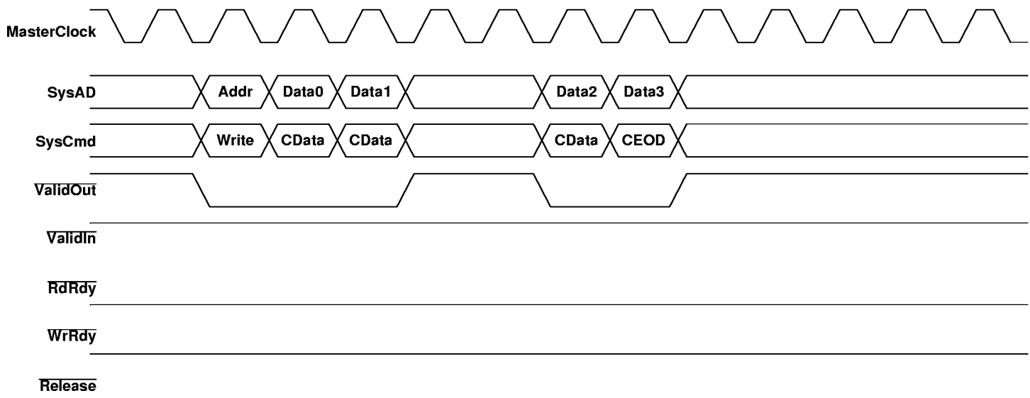
Figure 6: R4650 Block Write Request (64-bit system interface)
