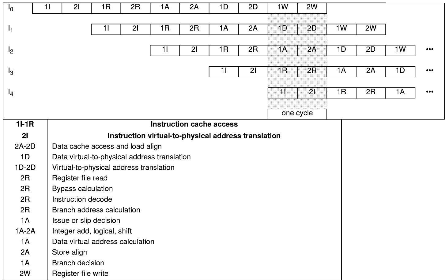
Figure 2: R4650 Pipeline
