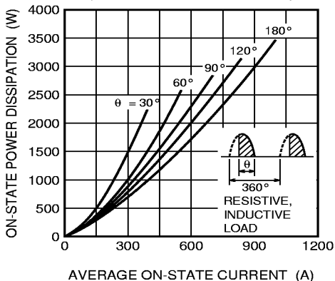
MAXIMUM ON-STATE POWER DISSIPATION CHARACTERISTICS (SINGLE-PHASE HALF WAVE)
