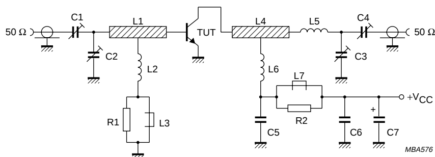
Fig.6 Class-B test circuit at f = 470 MHz.
