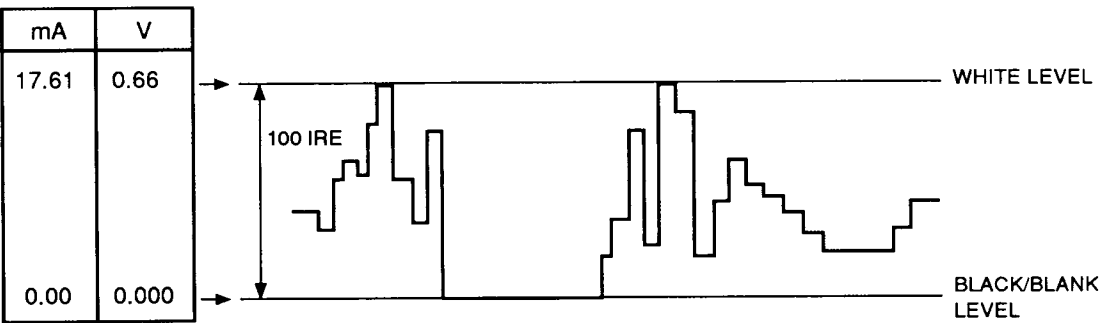
Figure 3. Composite Video Output Waveforms
