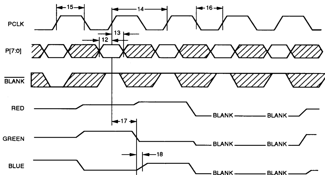
Figure 9. Pixel and Video Control Timing
