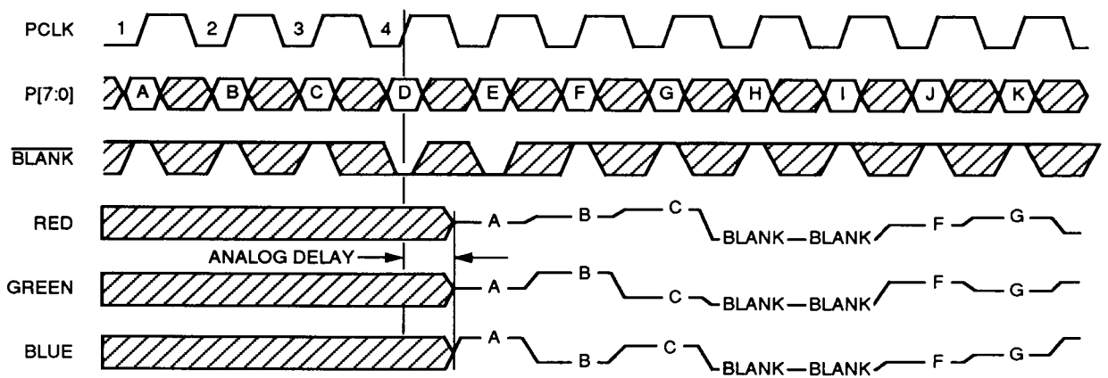
Figure 10. System Timing Diagram: Pixel Pipeline
