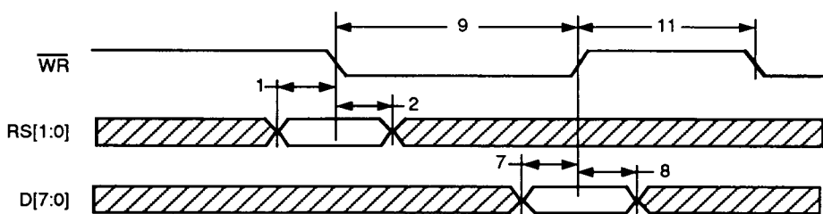
Figure 8. Basic Write-Cycle Timing Diagram
