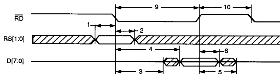
Figure 7. Basic Read-Cycle Timing Diagram
