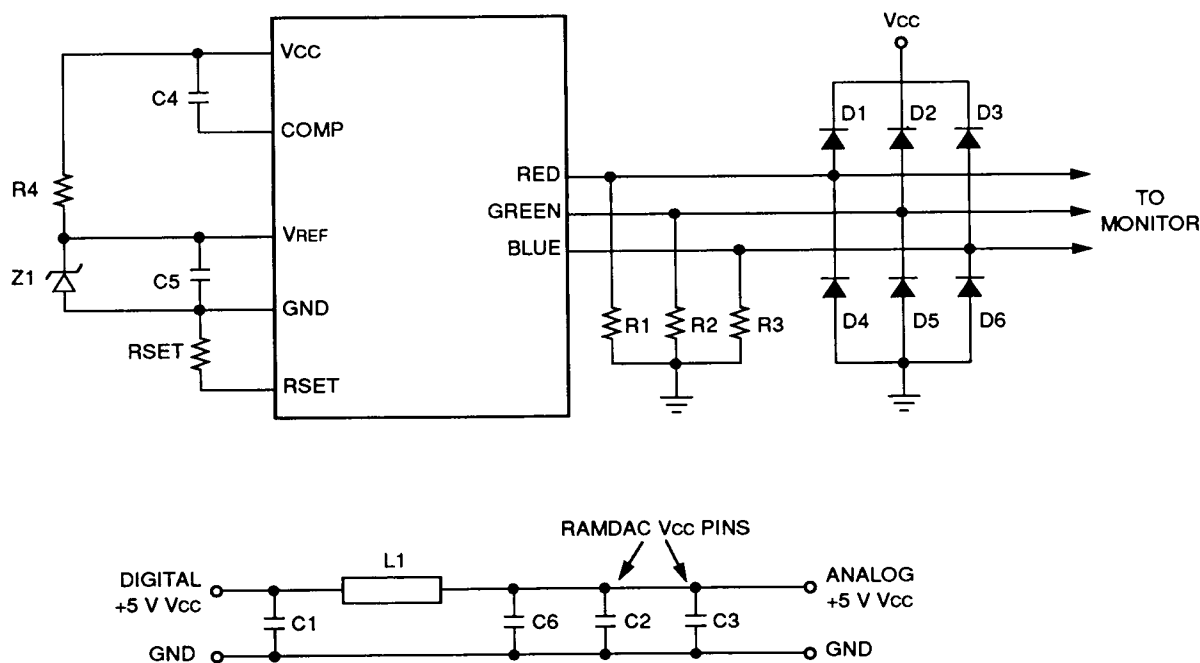
Figure 6. Typical Connection Diagram for External Voltage Reference
