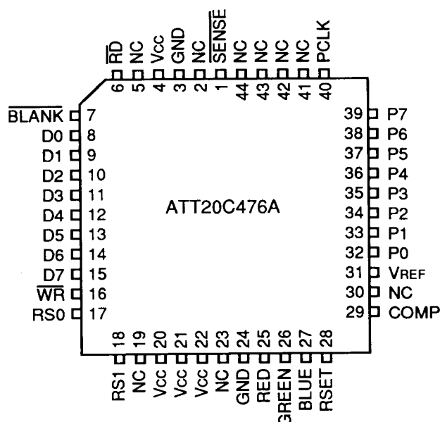
Figure 2. ATT20C476A Pin Diagram
