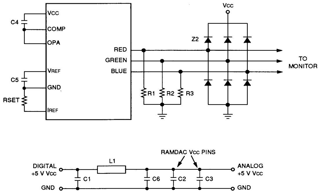
Figure 5. Typical Connection Diagram for Internal Voltage Reference
