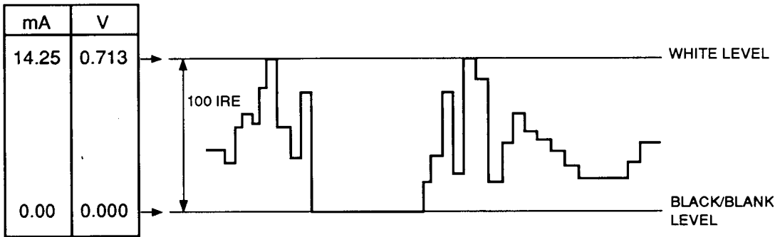
Figure 4. PS/2 Composite Video Output Waveforms
