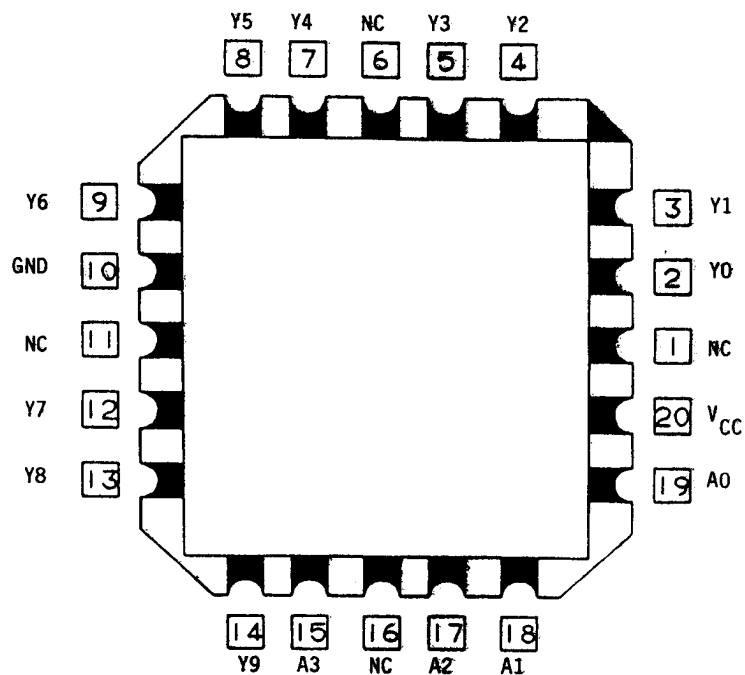
FIGURE 1. Terminal connections.
