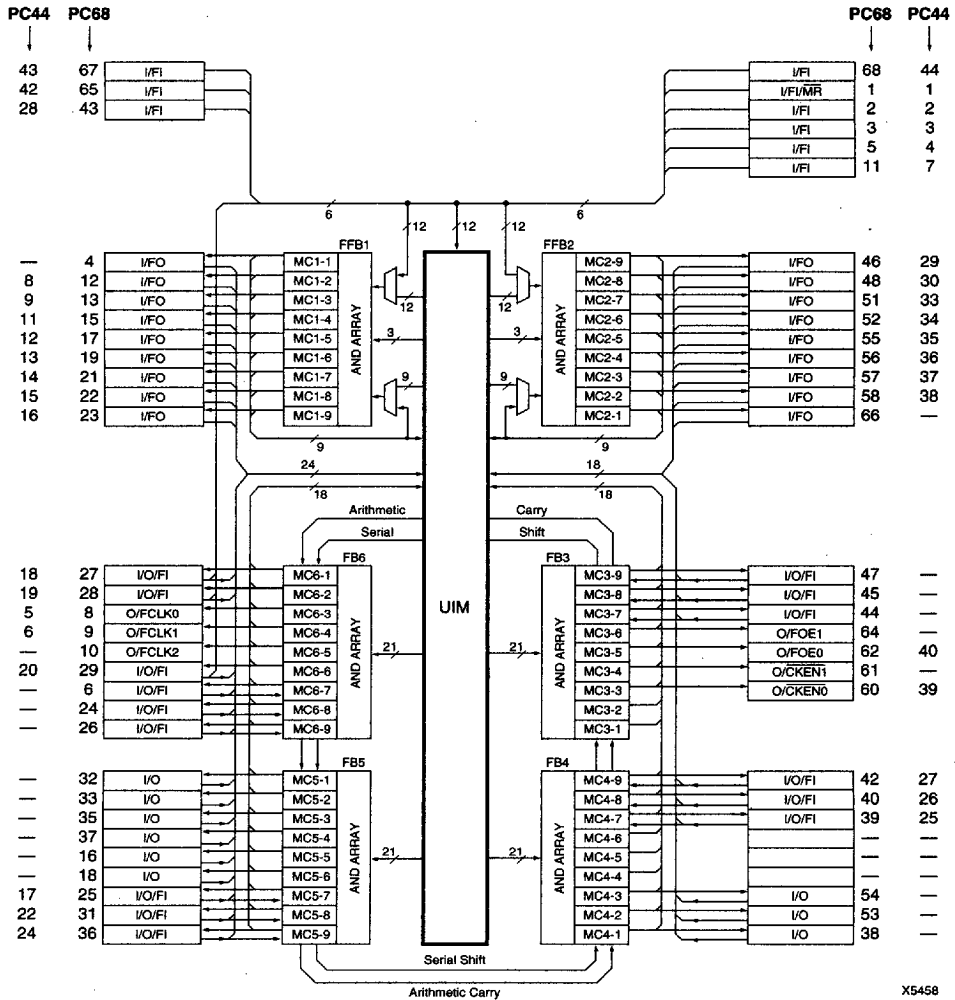
Figure 2: XC7354 Architecture
