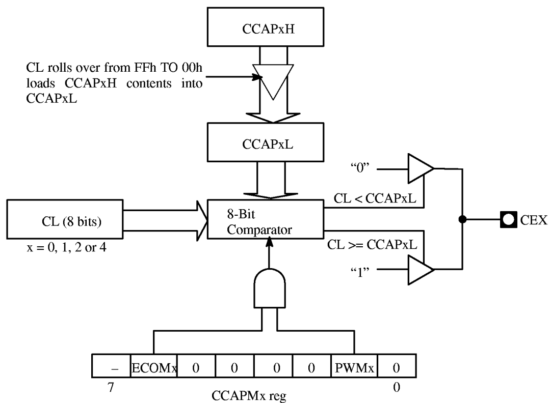
Figure 5.5. PWM Mode
