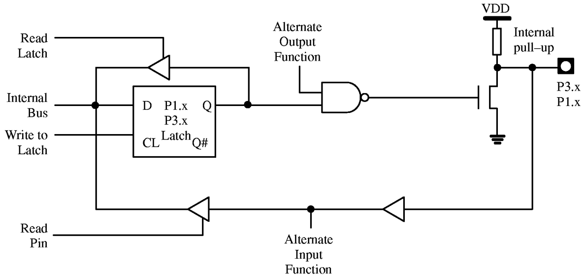
Figure 2.1. Port 1 and Port 3 Structure
