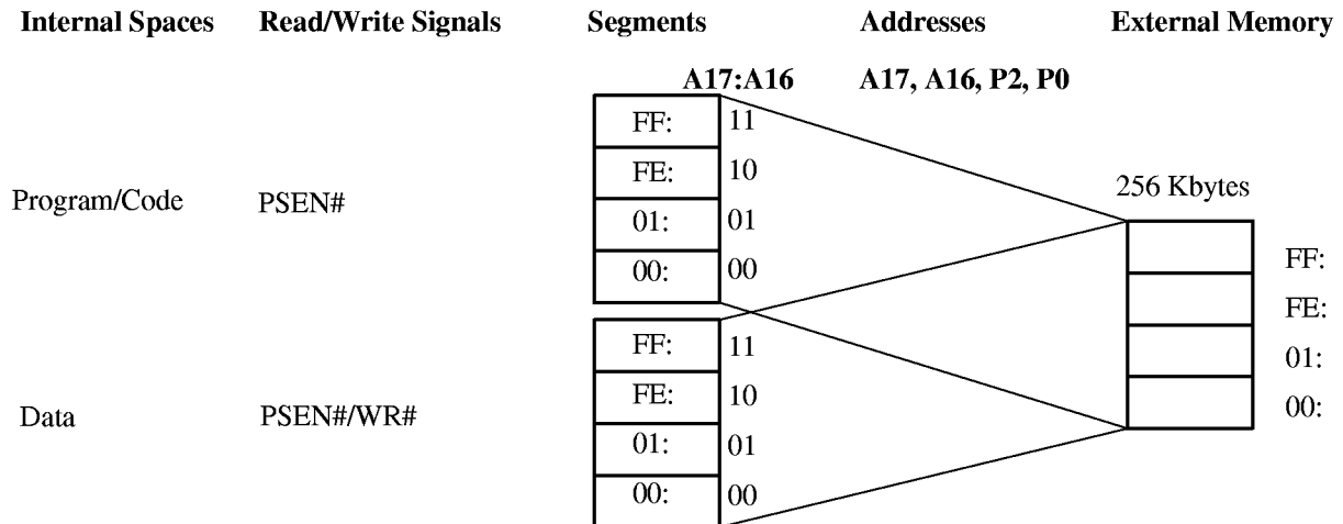
Figure 1.5. Internal/External Memory Segments (RD1:0 = 00)
