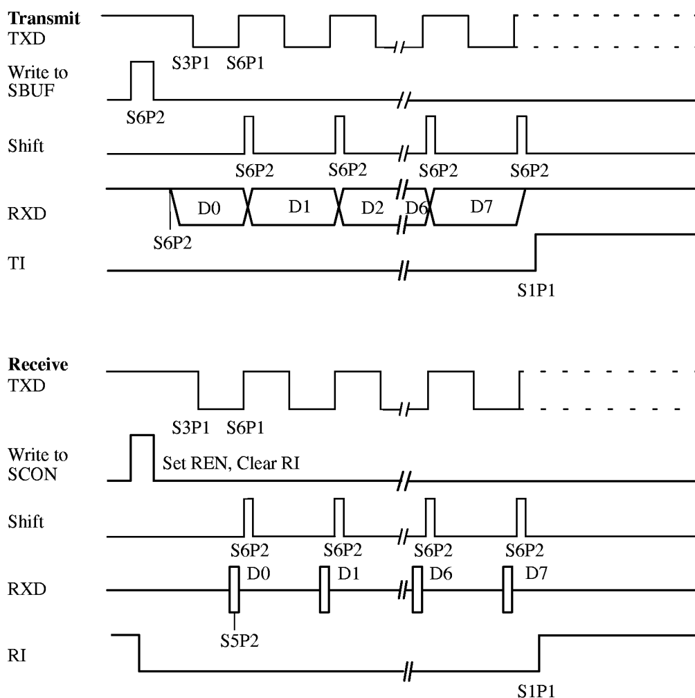
Figure 4.2. Mode 0 Timings
