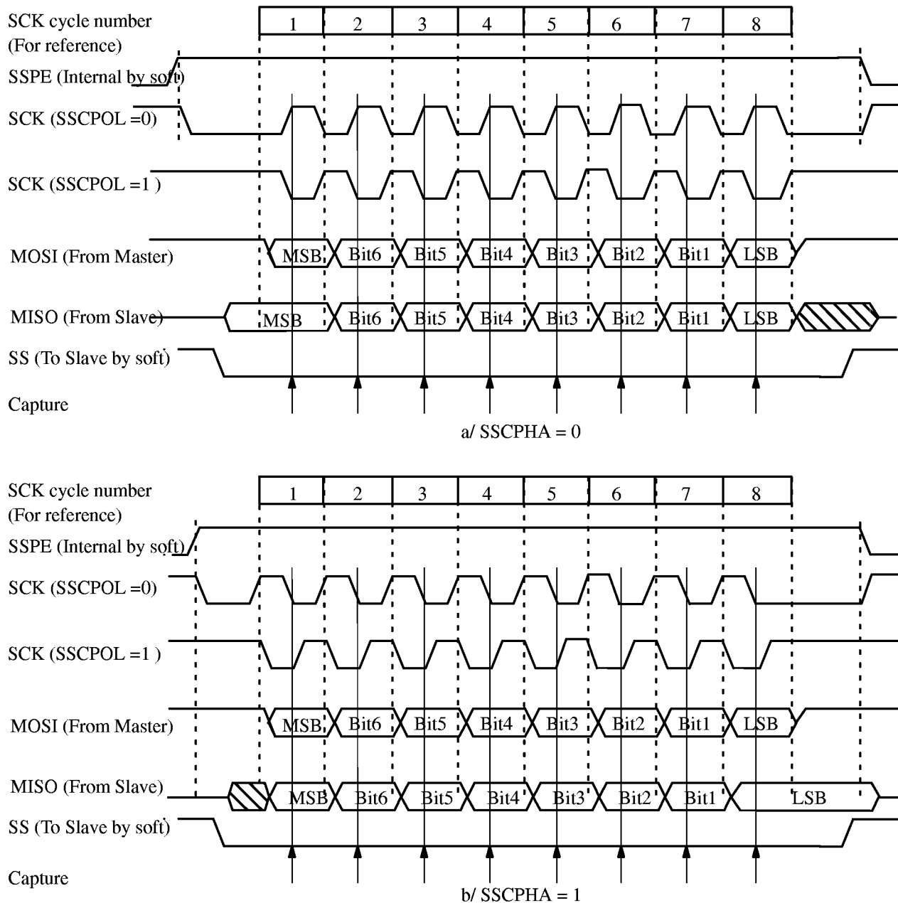
Figure 7.3. Data Transmission (a/ SSCPCHA = 0, b/ SSCPCHA = 1)
