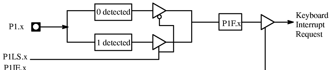
Figure 10.2. Keyboard Interface Interrupt Structure
