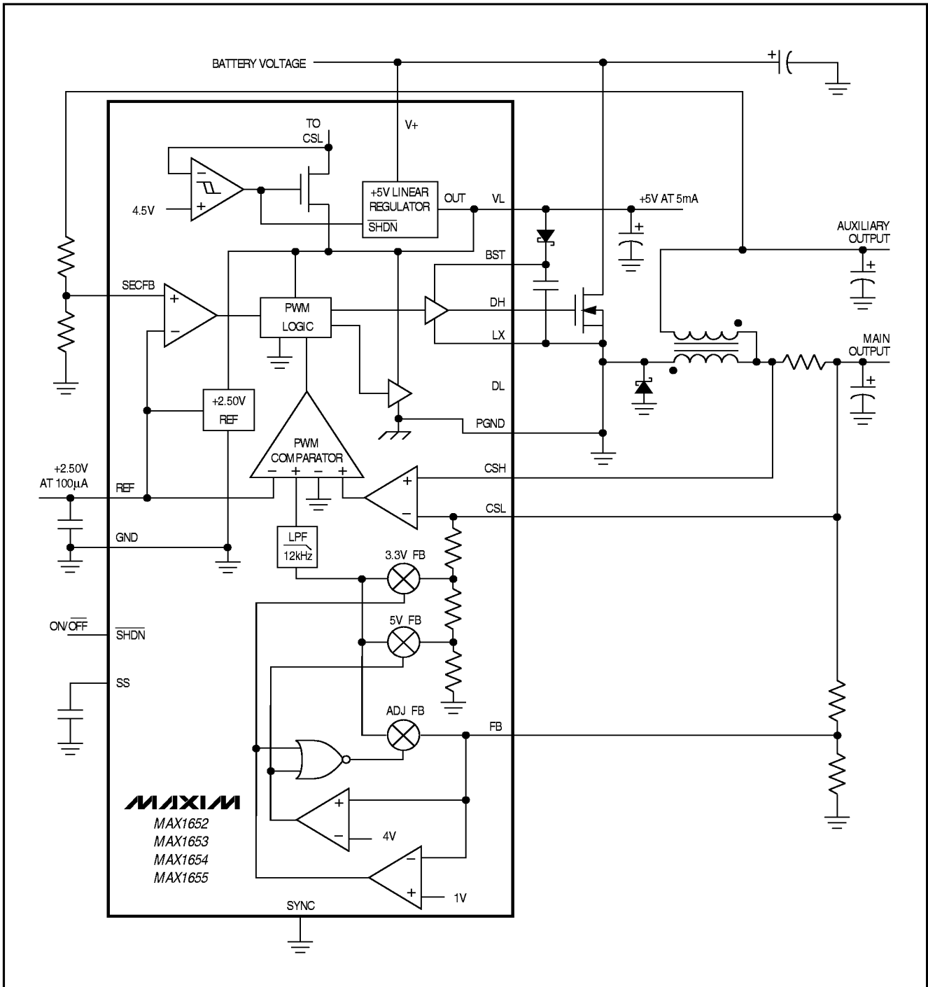
Figure 2. MAX1652-MAX1655 Functional Diagram
