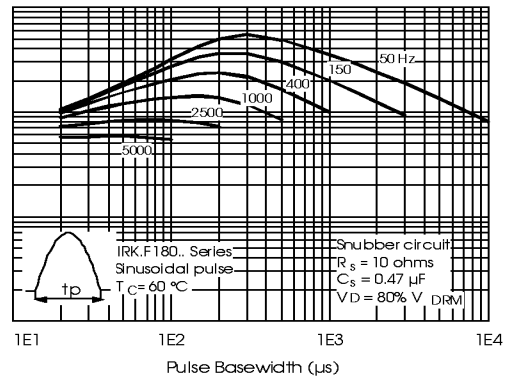
Fig. 11 - Frequency Characteristics
