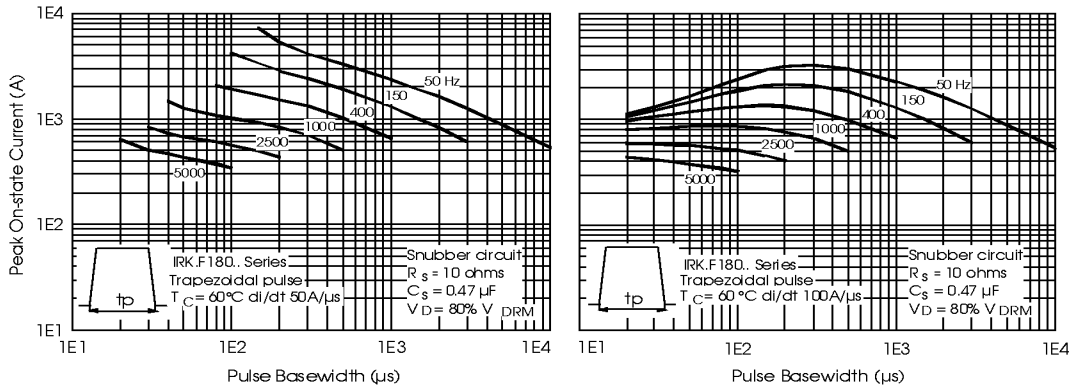
Fig. 13 - Frequency Characteristics
