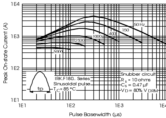
Fig. 11 - Frequency Characteristics
