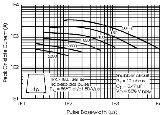
Fig. 12 - Frequency Characteristics
