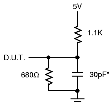
Figure 1. Output Load
